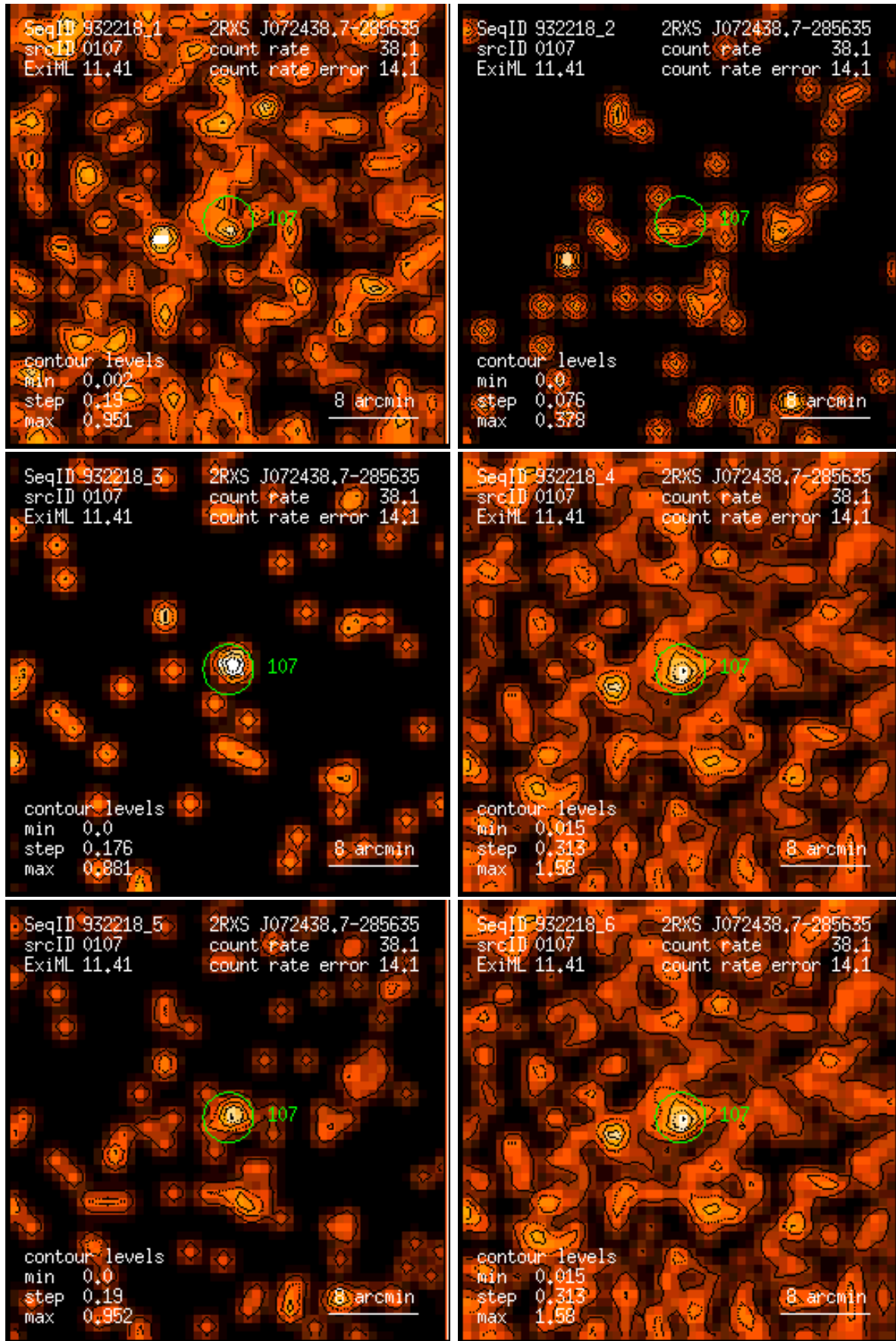
Figure 107: RASS 932218: detection 0107: band rate images, Gaussian filter: (1) PSPC channels 11 – 41, (2) 52 – 90, (3) 91 – 201, (4) 11 – 235, (5) 52 – 201, (6) 11 – 201. Broad band rates in counts/ks. Band rate contour levels in counts/ks/arcmin 2 .
