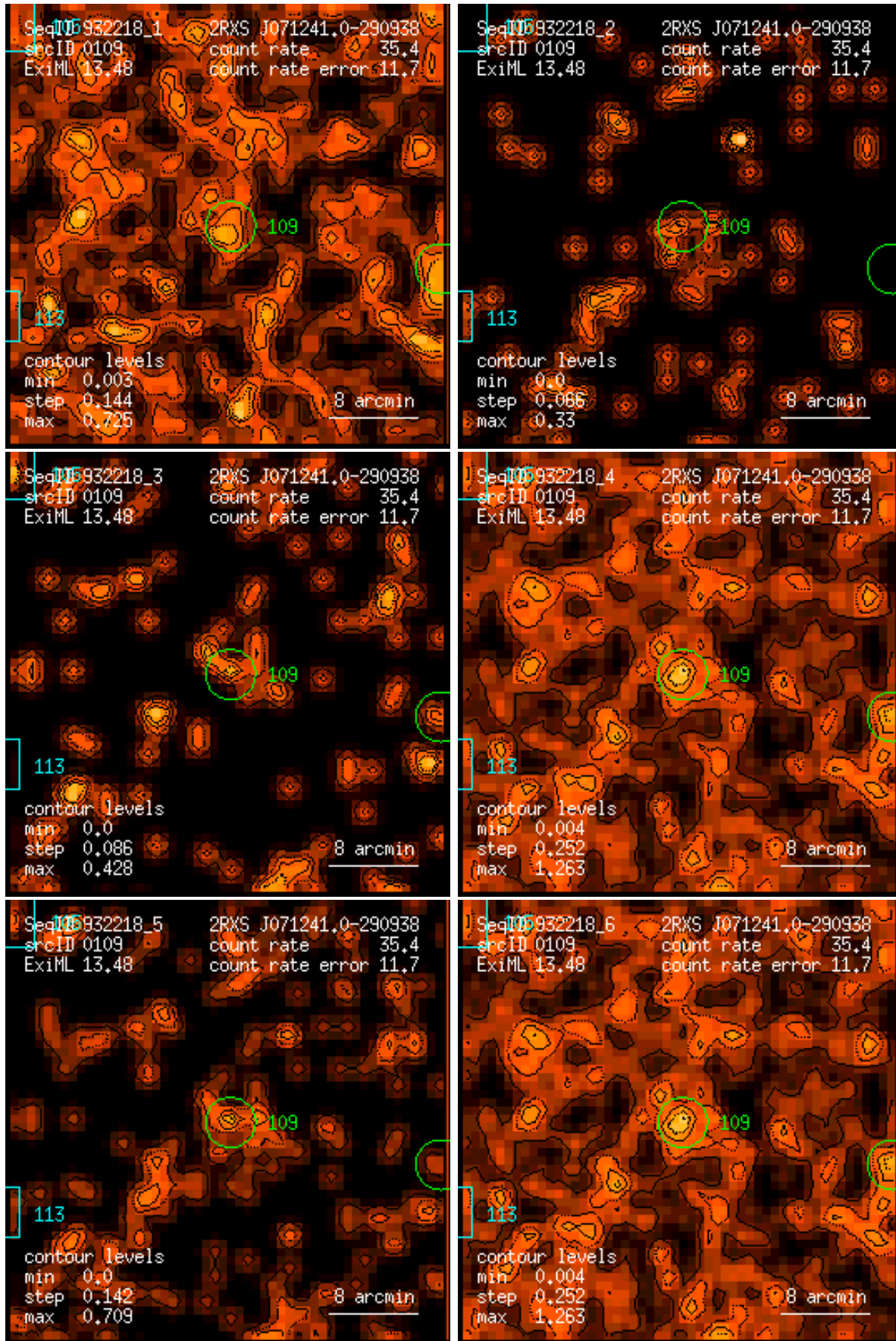
Figure 109: RASS 932218: detection 0109: band rate images, Gaussian filter: (1) PSPC channels 11 – 41, (2) 52 – 90, (3) 91 – 201, (4) 11 – 235, (5) 52 – 201, (6) 11 – 201. Broad band rates in counts/ks. Band rate contour levels in counts/ks/arcmin 2 .
