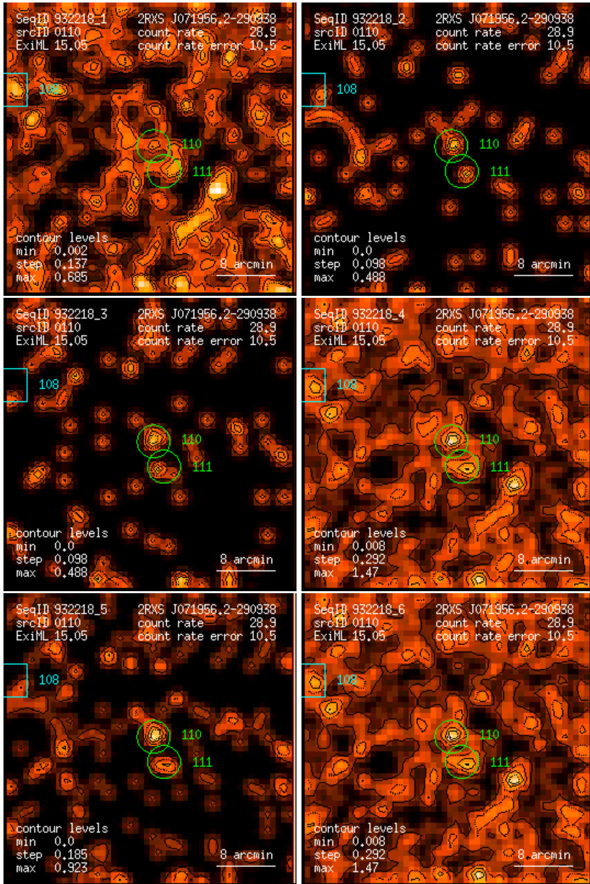
Figure 110: RASS 932218: detection 0110: band rate images, Gaussian filter: (1) PSPC channels 11 – 41, (2) 52 – 90, (3) 91 – 201, (4) 11 – 235, (5) 52 – 201, (6) 11 – 201. Broad band rates in counts/ks. Band rate contour levels in counts/ks/arcmin 2 .
