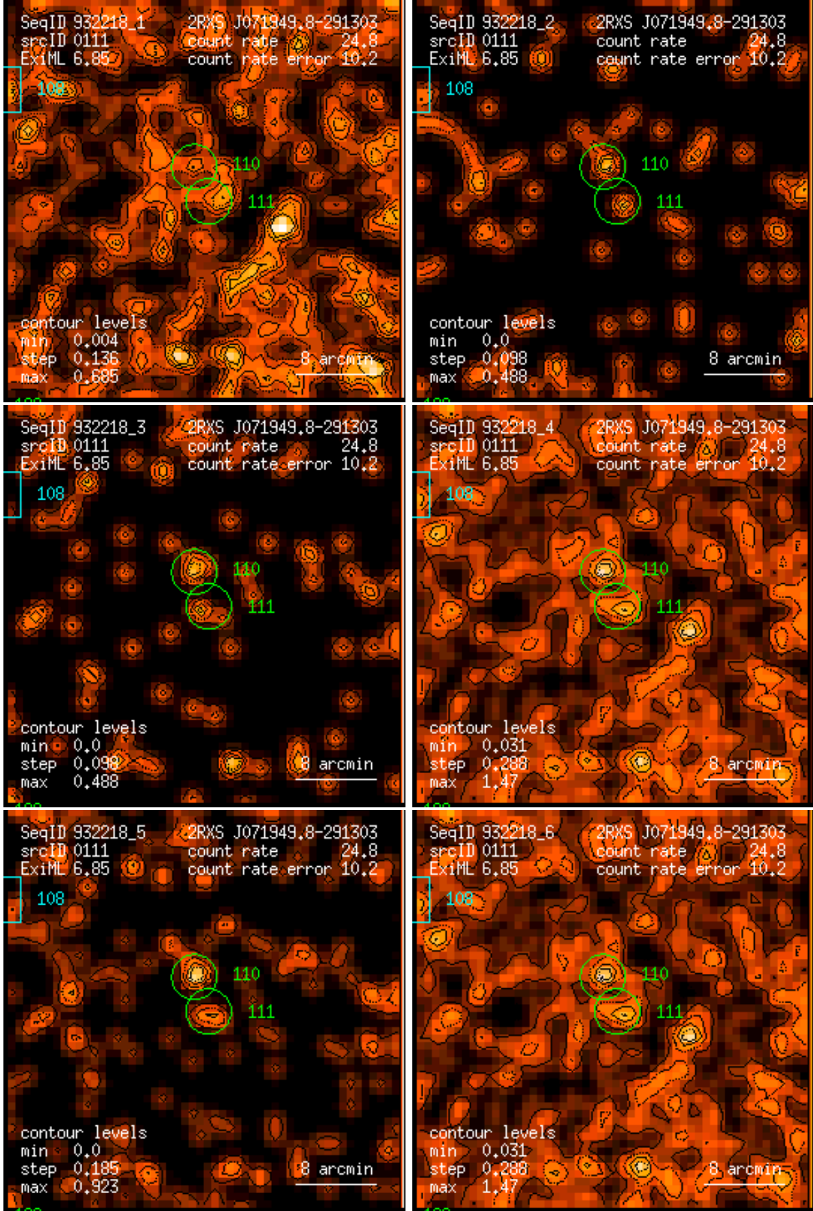
Figure 111: RASS 932218: detection 0111: band rate images, Gaussian filter: (1) PSPC channels 11 – 41, (2) 52 – 90, (3) 91 – 201, (4) 11 – 235, (5) 52 – 201, (6) 11 – 201. Broad band rates in counts/ks. Band rate contour levels in counts/ks/arcmin 2 .
