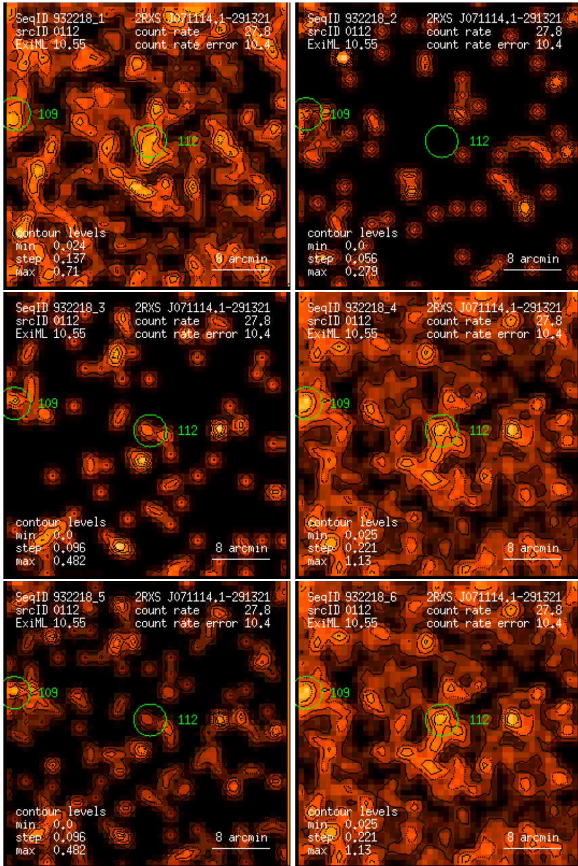
Figure 112: RASS 932218: detection 0112: band rate images, Gaussian filter: (1) PSPC channels 11 – 41, (2) 52 – 90, (3) 91 – 201, (4) 11 – 235, (5) 52 – 201, (6) 11 – 201. Broad band rates in counts/ks. Band rate contour levels in counts/ks/arcmin 2 .
