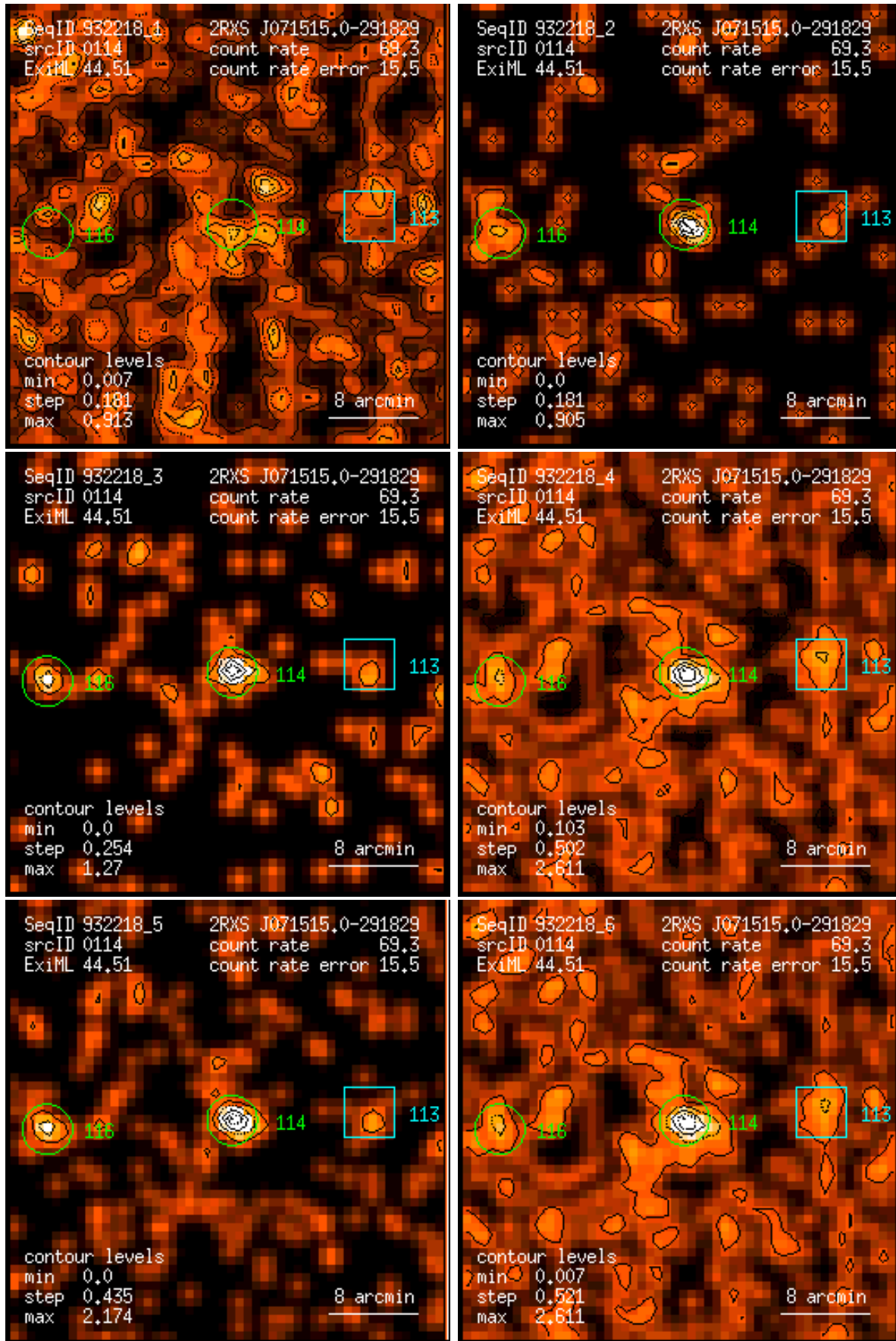
Figure 114: RASS 932218: detection 0114: band rate images, Gaussian filter: (1) PSPC channels 11 – 41, (2) 52 – 90, (3) 91 – 201, (4) 11 – 235, (5) 52 – 201, (6) 11 – 201. Broad band rates in counts/ks. Band rate contour levels in counts/ks/arcmin 2 .
