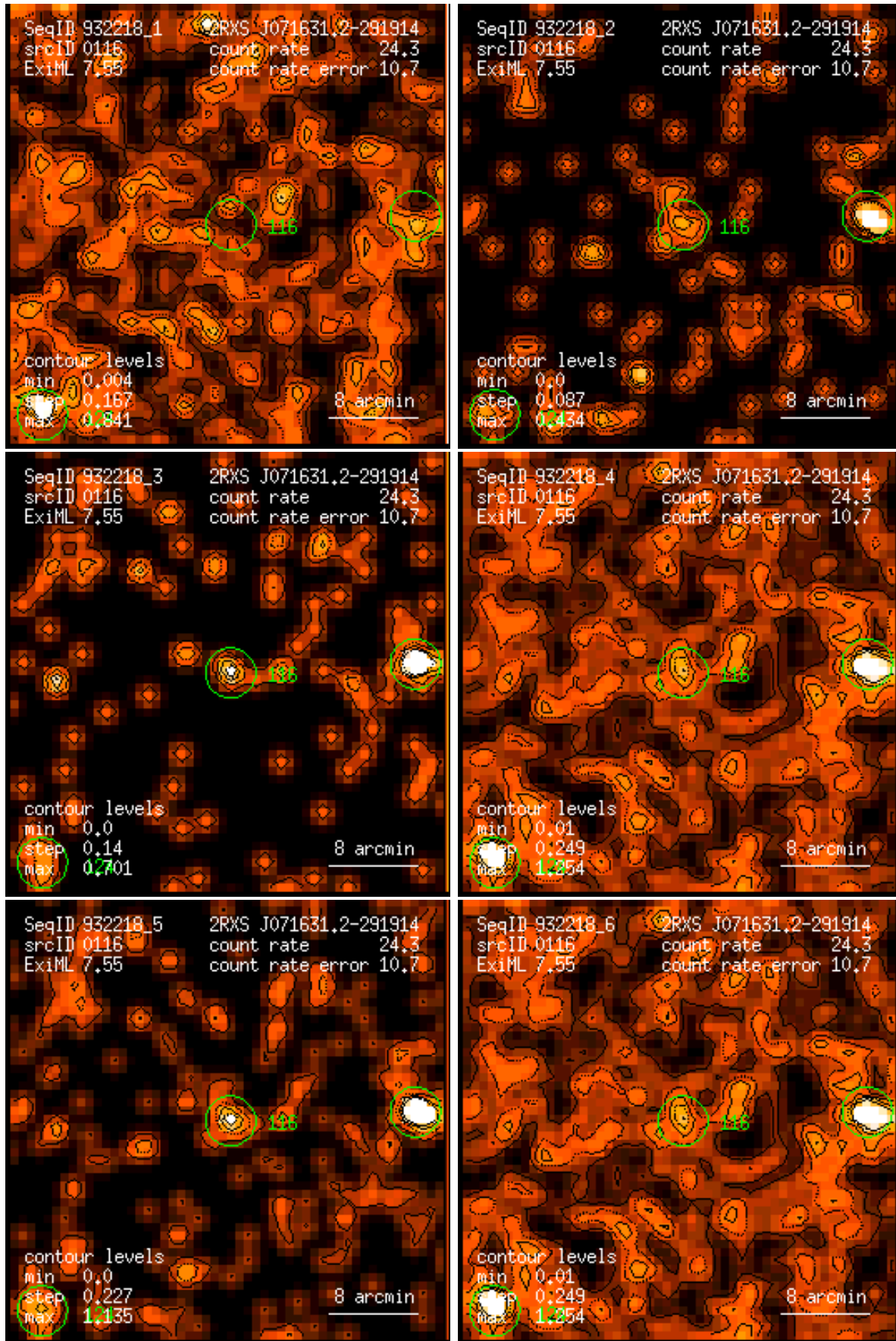
Figure 116: RASS 932218: detection 0116: band rate images, Gaussian filter: (1) PSPC channels 11 – 41, (2) 52 – 90, (3) 91 – 201, (4) 11 – 235, (5) 52 – 201, (6) 11 – 201. Broad band rates in counts/ks. Band rate contour levels in counts/ks/arcmin 2 .
