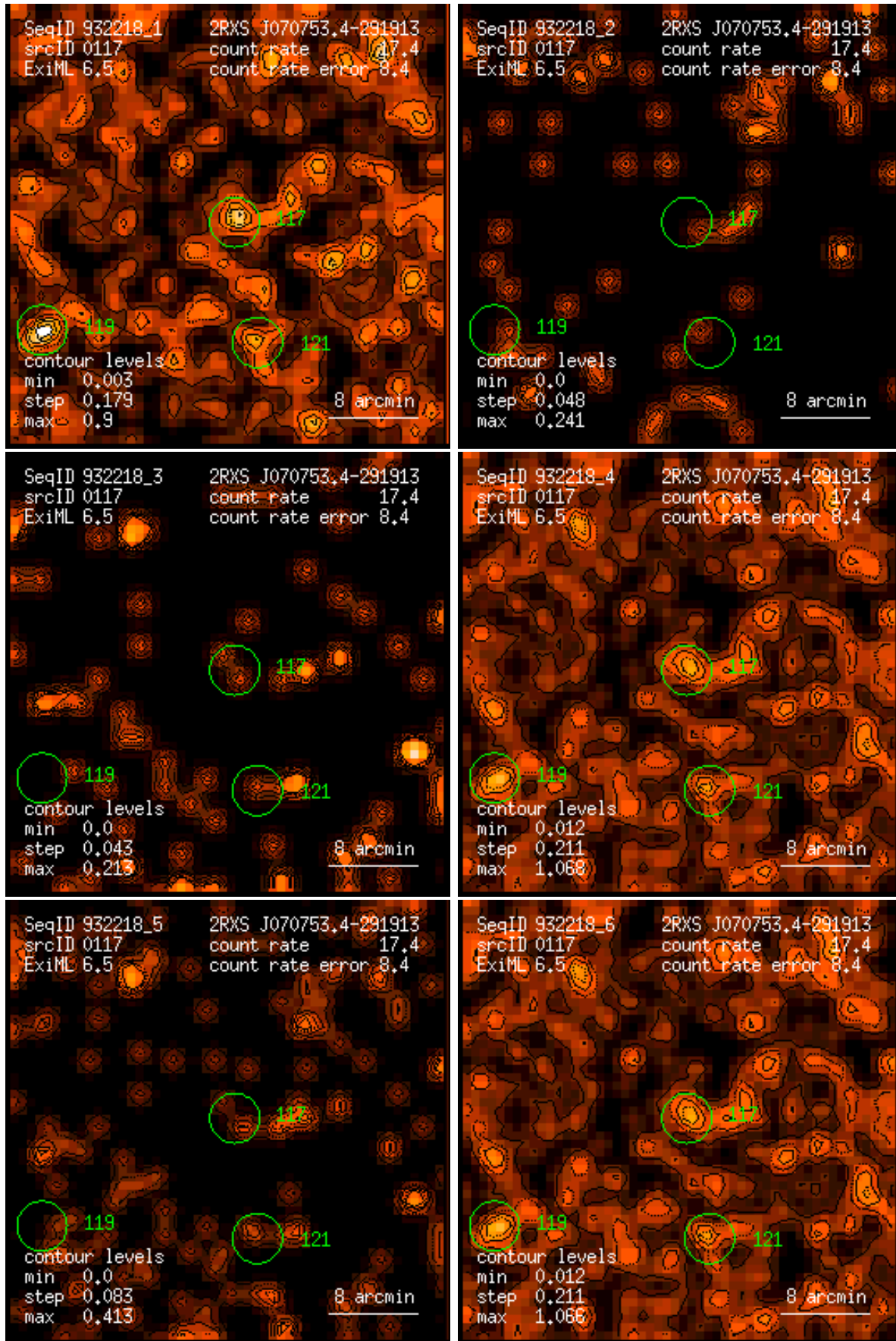
Figure 117: RASS 932218: detection 0117: band rate images, Gaussian filter: (1) PSPC channels 11 – 41, (2) 52 – 90, (3) 91 – 201, (4) 11 – 235, (5) 52 – 201, (6) 11 – 201. Broad band rates in counts/ks. Band rate contour levels in counts/ks/arcmin 2 .
