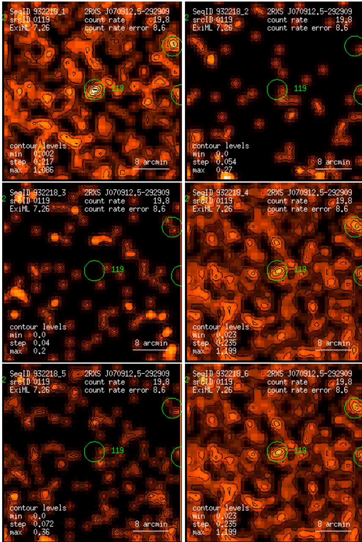
Figure 119: RASS 932218: detection 0119: band rate images, Gaussian filter: (1) PSPC channels 11 – 41, (2) 52 – 90, (3) 91 – 201, (4) 11 – 235, (5) 52 – 201, (6) 11 – 201. Broad band rates in counts/ks. Band rate contour levels in counts/ks/arcmin 2 .
