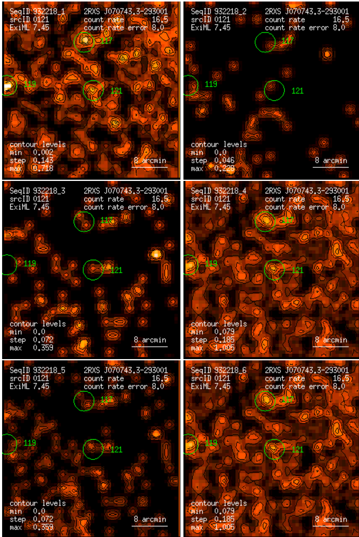
Figure 121: RASS 932218: detection 0121: band rate images, Gaussian filter: (1) PSPC channels 11 – 41, (2) 52 – 90, (3) 91 – 201, (4) 11 – 235, (5) 52 – 201, (6) 11 – 201. Broad band rates in counts/ks. Band rate contour levels in counts/ks/arcmin 2 .
