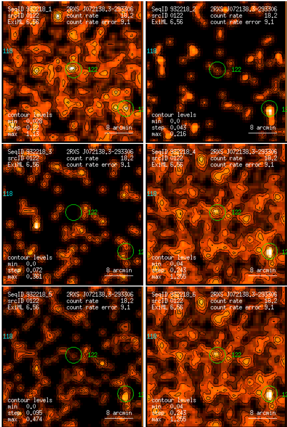
Figure 122: RASS 932218: detection 0122: band rate images, Gaussian filter: (1) PSPC channels 11 – 41, (2) 52 – 90, (3) 91 – 201, (4) 11 – 235, (5) 52 – 201, (6) 11 – 201. Broad band rates in counts/ks. Band rate contour levels in counts/ks/arcmin 2 .
