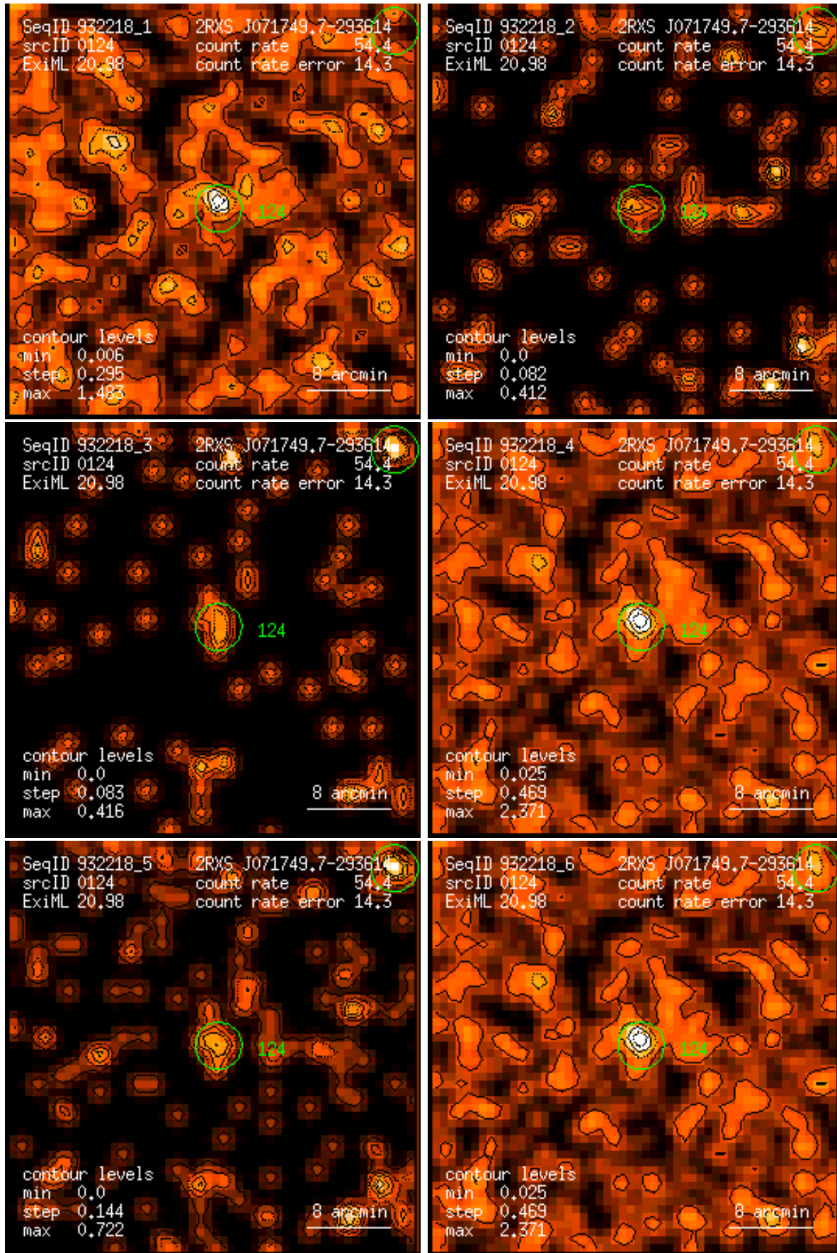
Figure 124: RASS 932218: detection 0124: band rate images, Gaussian filter: (1) PSPC channels 11 – 41, (2) 52 – 90, (3) 91 – 201, (4) 11 – 235, (5) 52 – 201, (6) 11 – 201. Broad band rates in counts/ks. Band rate contour levels in counts/ks/arcmin 2 .
