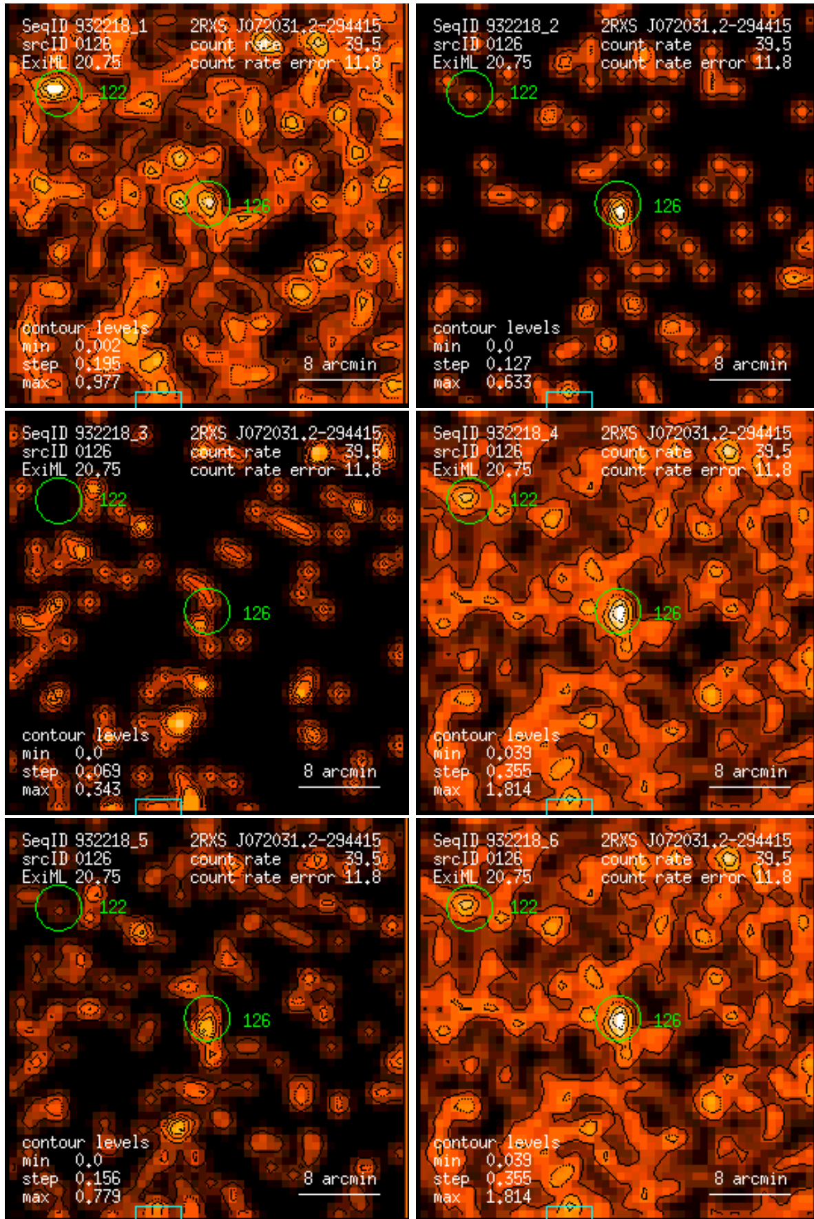
Figure 126: RASS 932218: detection 0126: band rate images, Gaussian filter: (1) PSPC channels 11 – 41, (2) 52 – 90, (3) 91 – 201, (4) 11 – 235, (5) 52 – 201, (6) 11 – 201. Broad band rates in counts/ks. Band rate contour levels in counts/ks/arcmin 2 .
