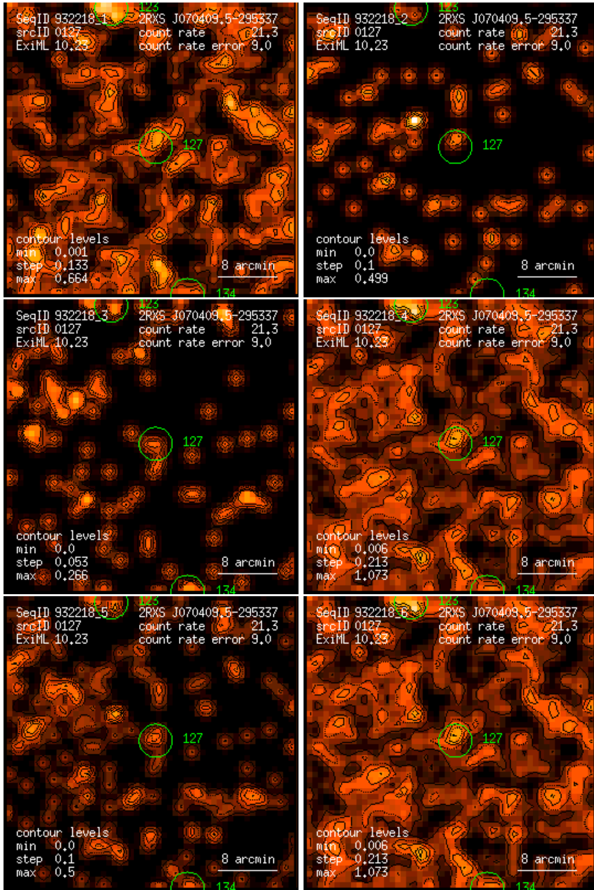
Figure 127: RASS 932218: detection 0127: band rate images, Gaussian filter: (1) PSPC channels 11 – 41, (2) 52 – 90, (3) 91 – 201, (4) 11 – 235, (5) 52 – 201, (6) 11 – 201. Broad band rates in counts/ks. Band rate contour levels in counts/ks/arcmin 2 .
