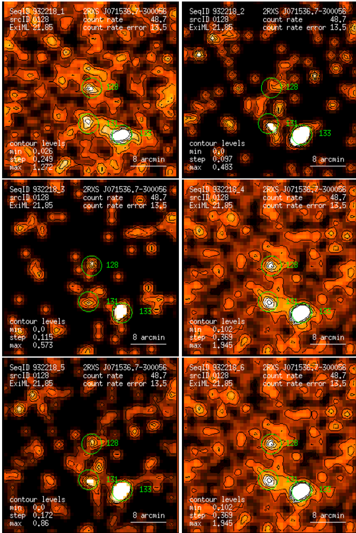
Figure 128: RASS 932218: detection 0128: band rate images, Gaussian filter: (1) PSPC channels 11 – 41, (2) 52 – 90, (3) 91 – 201, (4) 11 – 235, (5) 52 – 201, (6) 11 – 201. Broad band rates in counts/ks. Band rate contour levels in counts/ks/arcmin 2 .
