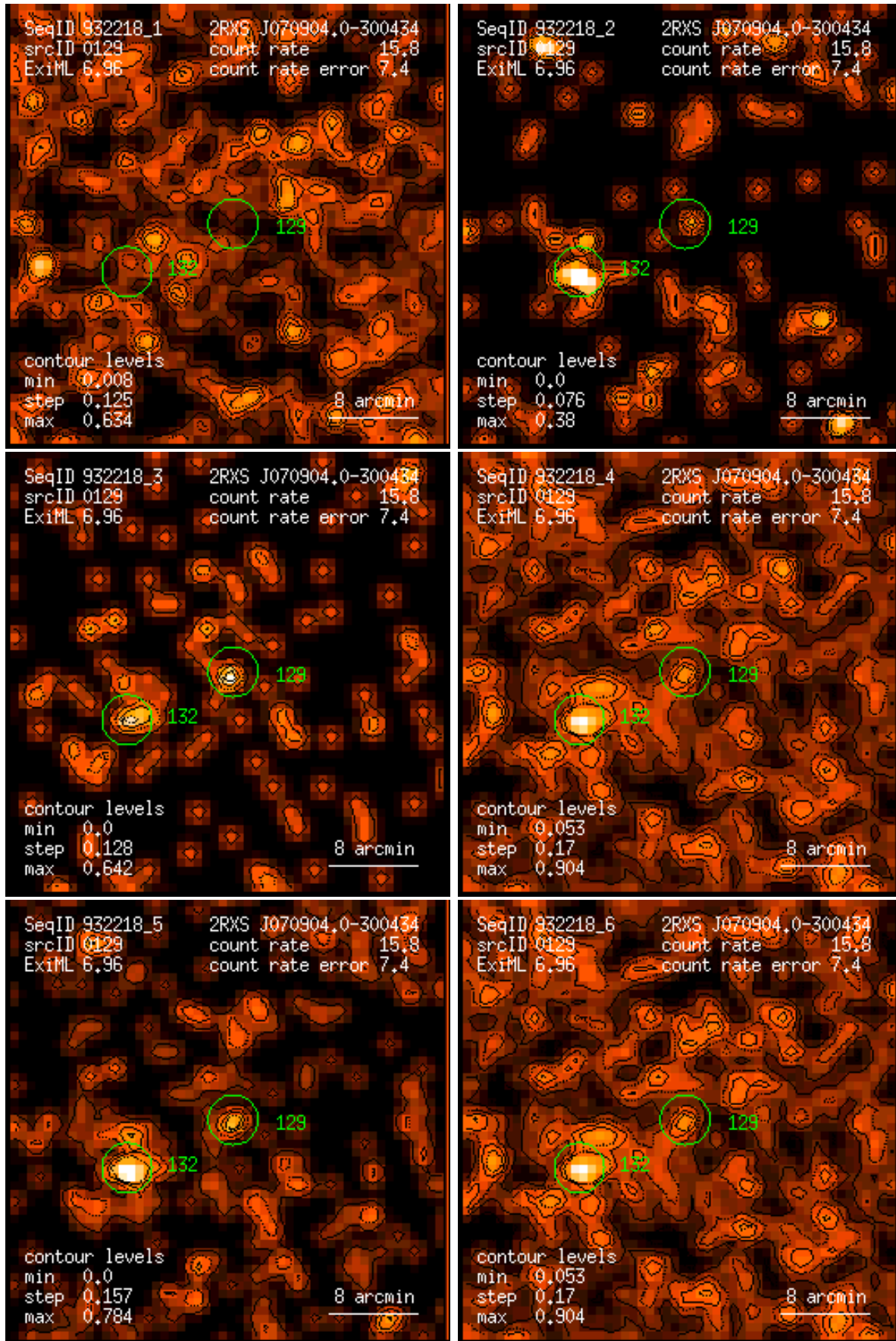
Figure 129: RASS 932218: detection 0129: band rate images, Gaussian filter: (1) PSPC channels 11 – 41, (2) 52 – 90, (3) 91 – 201, (4) 11 – 235, (5) 52 – 201, (6) 11 – 201. Broad band rates in counts/ks. Band rate contour levels in counts/ks/arcmin 2 .
