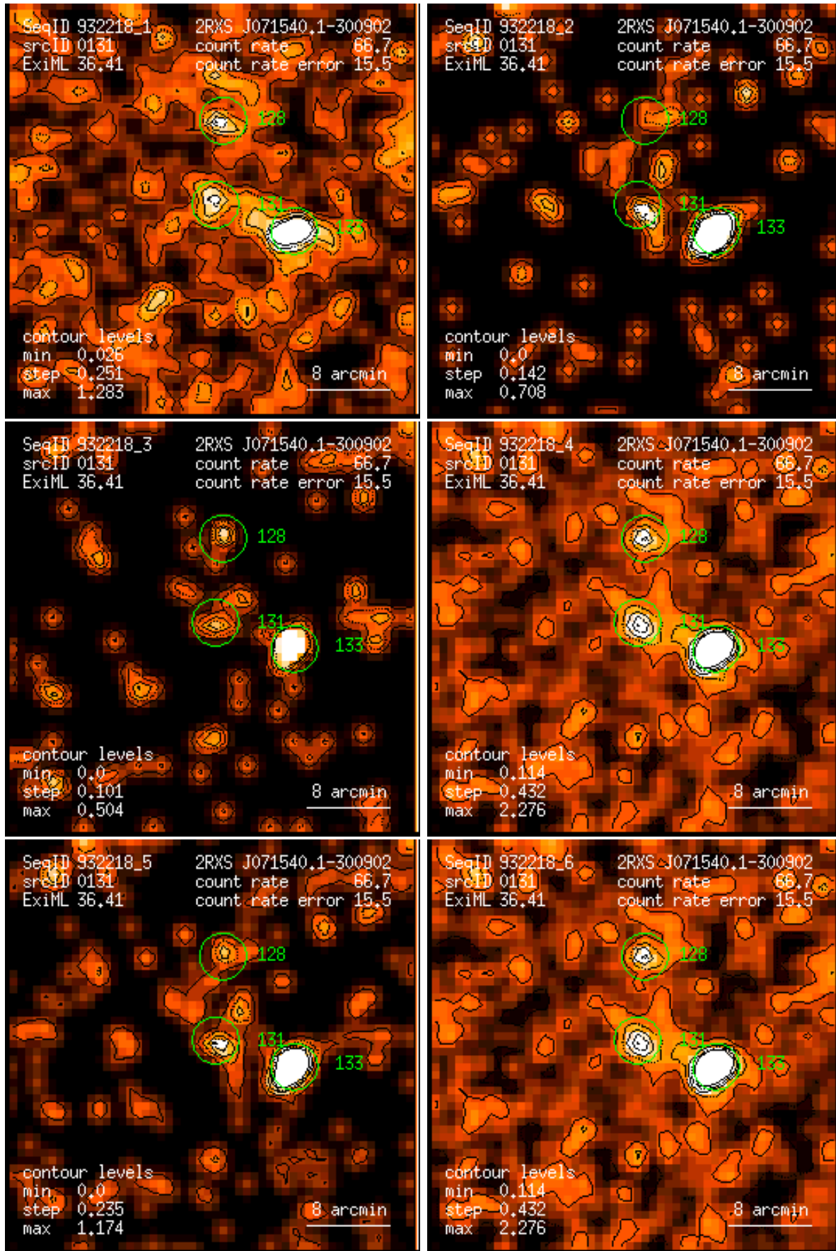
Figure 131: RASS 932218: detection 0131: band rate images, Gaussian filter: (1) PSPC channels 11 – 41, (2) 52 – 90, (3) 91 – 201, (4) 11 – 235, (5) 52 – 201, (6) 11 – 201. Broad band rates in counts/ks. Band rate contour levels in counts/ks/arcmin 2 .
