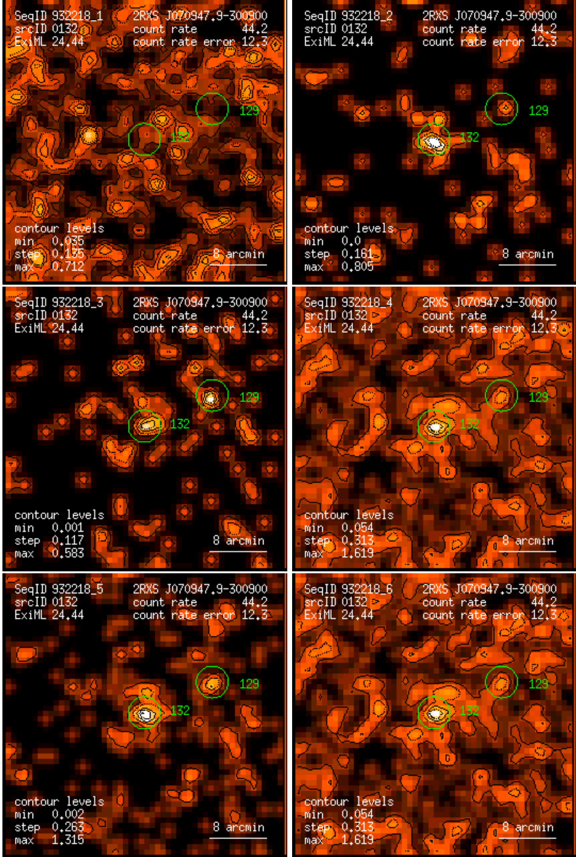
Figure 132: RASS 932218: detection 0132: band rate images, Gaussian filter: (1) PSPC channels 11 – 41, (2) 52 – 90, (3) 91 – 201, (4) 11 – 235, (5) 52 – 201, (6) 11 – 201. Broad band rates in counts/ks. Band rate contour levels in counts/ks/arcmin 2 .
