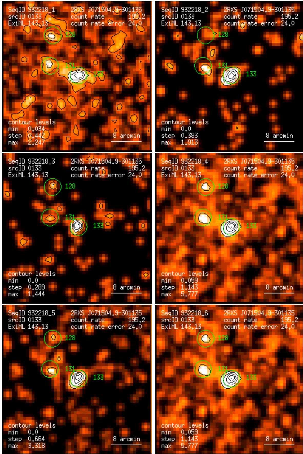
Figure 133: RASS 932218: detection 0133: band rate images, Gaussian filter: (1) PSPC channels 11 – 41, (2) 52 – 90, (3) 91 – 201, (4) 11 – 235, (5) 52 – 201, (6) 11 – 201. Broad band rates in counts/ks. Band rate contour levels in counts/ks/arcmin 2 .
