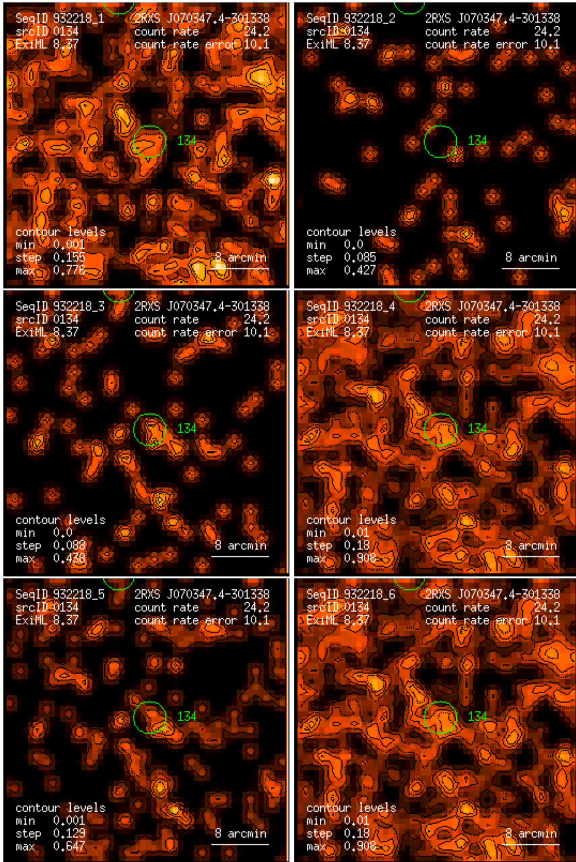
Figure 134: RASS 932218: detection 0134: band rate images, Gaussian filter: (1) PSPC channels 11 – 41, (2) 52 – 90, (3) 91 – 201, (4) 11 – 235, (5) 52 – 201, (6) 11 – 201. Broad band rates in counts/ks. Band rate contour levels in counts/ks/arcmin 2 .
