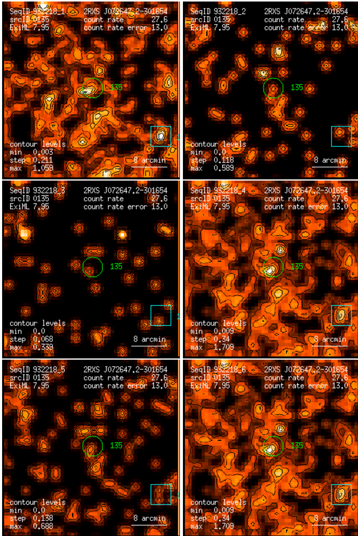
Figure 135: RASS 932218: detection 0135: band rate images, Gaussian filter: (1) PSPC channels 11 – 41, (2) 52 – 90, (3) 91 – 201, (4) 11 – 235, (5) 52 – 201, (6) 11 – 201. Broad band rates in counts/ks. Band rate contour levels in counts/ks/arcmin 2 .
