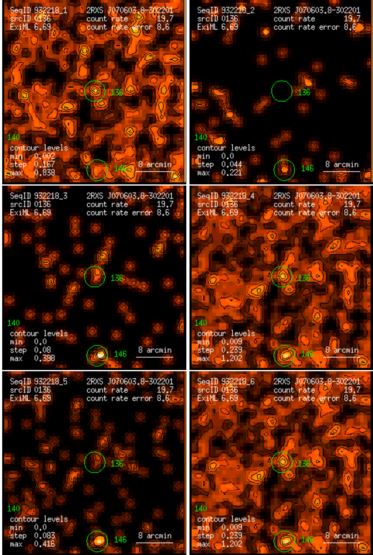
Figure 136: RASS 932218: detection 0136: band rate images, Gaussian filter: (1) PSPC channels 11 – 41, (2) 52 – 90, (3) 91 – 201, (4) 11 – 235, (5) 52 – 201, (6) 11 – 201. Broad band rates in counts/ks. Band rate contour levels in counts/ks/arcmin 2 .
