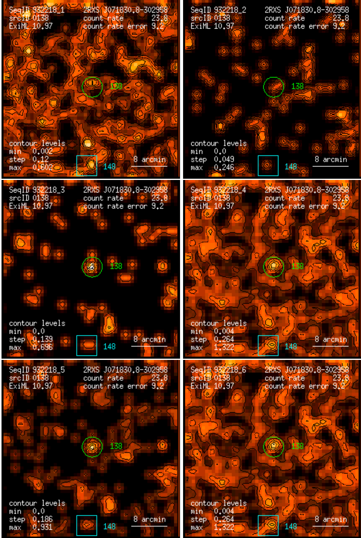
Figure 138: RASS 932218: detection 0138: band rate images, Gaussian filter: (1) PSPC channels 11 – 41, (2) 52 – 90, (3) 91 – 201, (4) 11 – 235, (5) 52 – 201, (6) 11 – 201. Broad band rates in counts/ks. Band rate contour levels in counts/ks/arcmin 2 .
