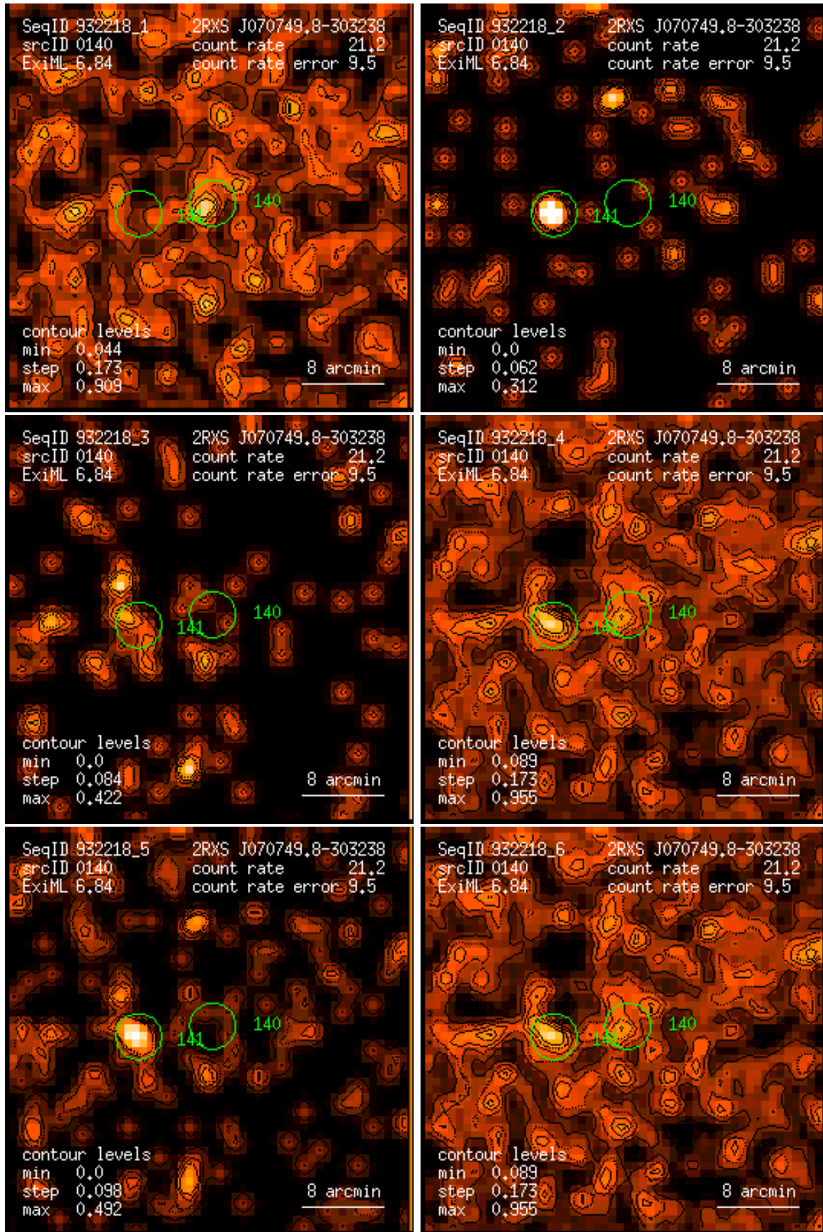
Figure 140: RASS 932218: detection 0140: band rate images, Gaussian filter: (1) PSPC channels 11 – 41, (2) 52 – 90, (3) 91 – 201, (4) 11 – 235, (5) 52 – 201, (6) 11 – 201. Broad band rates in counts/ks. Band rate contour levels in counts/ks/arcmin 2 .
