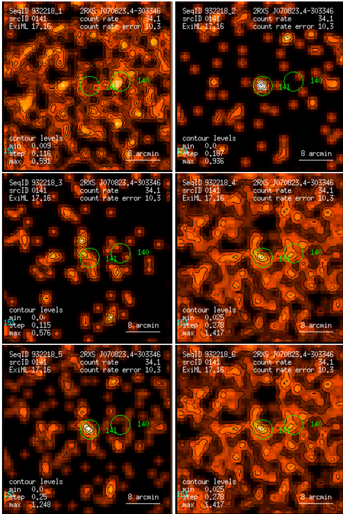
Figure 141: RASS 932218: detection 0141: band rate images, Gaussian filter: (1) PSPC channels 11 – 41, (2) 52 – 90, (3) 91 – 201, (4) 11 – 235, (5) 52 – 201, (6) 11 – 201. Broad band rates in counts/ks. Band rate contour levels in counts/ks/arcmin 2 .
