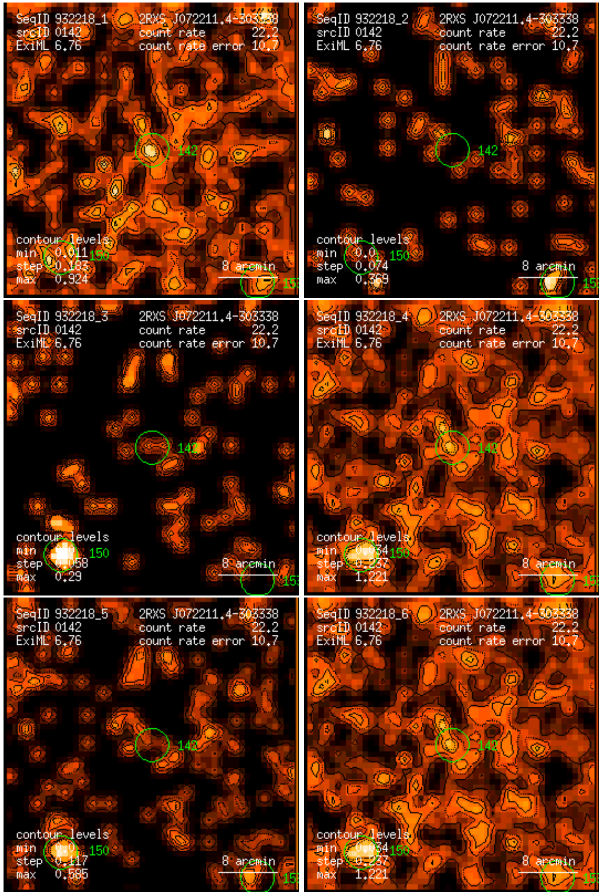
Figure 142: RASS 932218: detection 0142: band rate images, Gaussian filter: (1) PSPC channels 11 – 41, (2) 52 – 90, (3) 91 – 201, (4) 11 – 235, (5) 52 – 201, (6) 11 – 201. Broad band rates in counts/ks. Band rate contour levels in counts/ks/arcmin 2 .
