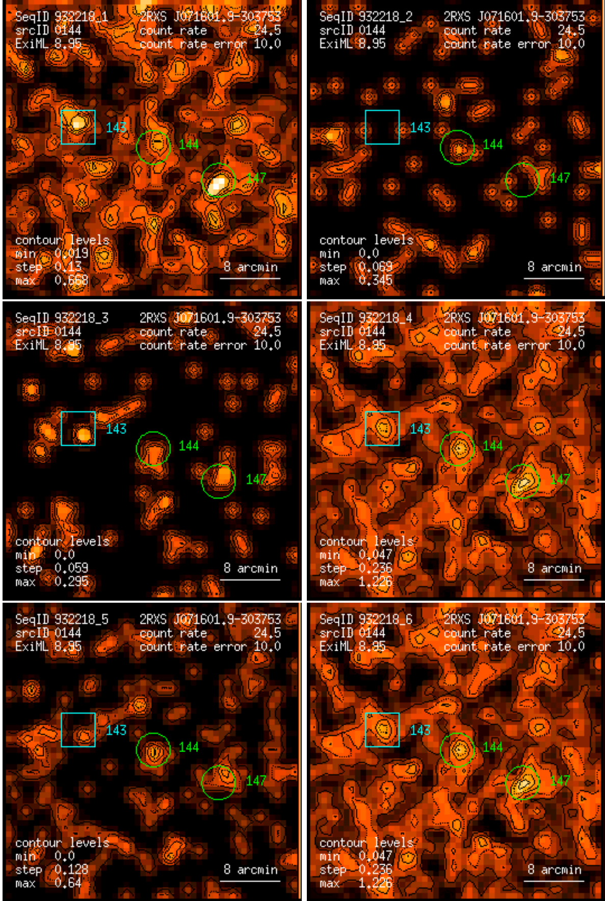
Figure 144: RASS 932218: detection 0144: band rate images, Gaussian filter: (1) PSPC channels 11 – 41, (2) 52 – 90, (3) 91 – 201, (4) 11 – 235, (5) 52 – 201, (6) 11 – 201. Broad band rates in counts/ks. Band rate contour levels in counts/ks/arcmin 2 .
