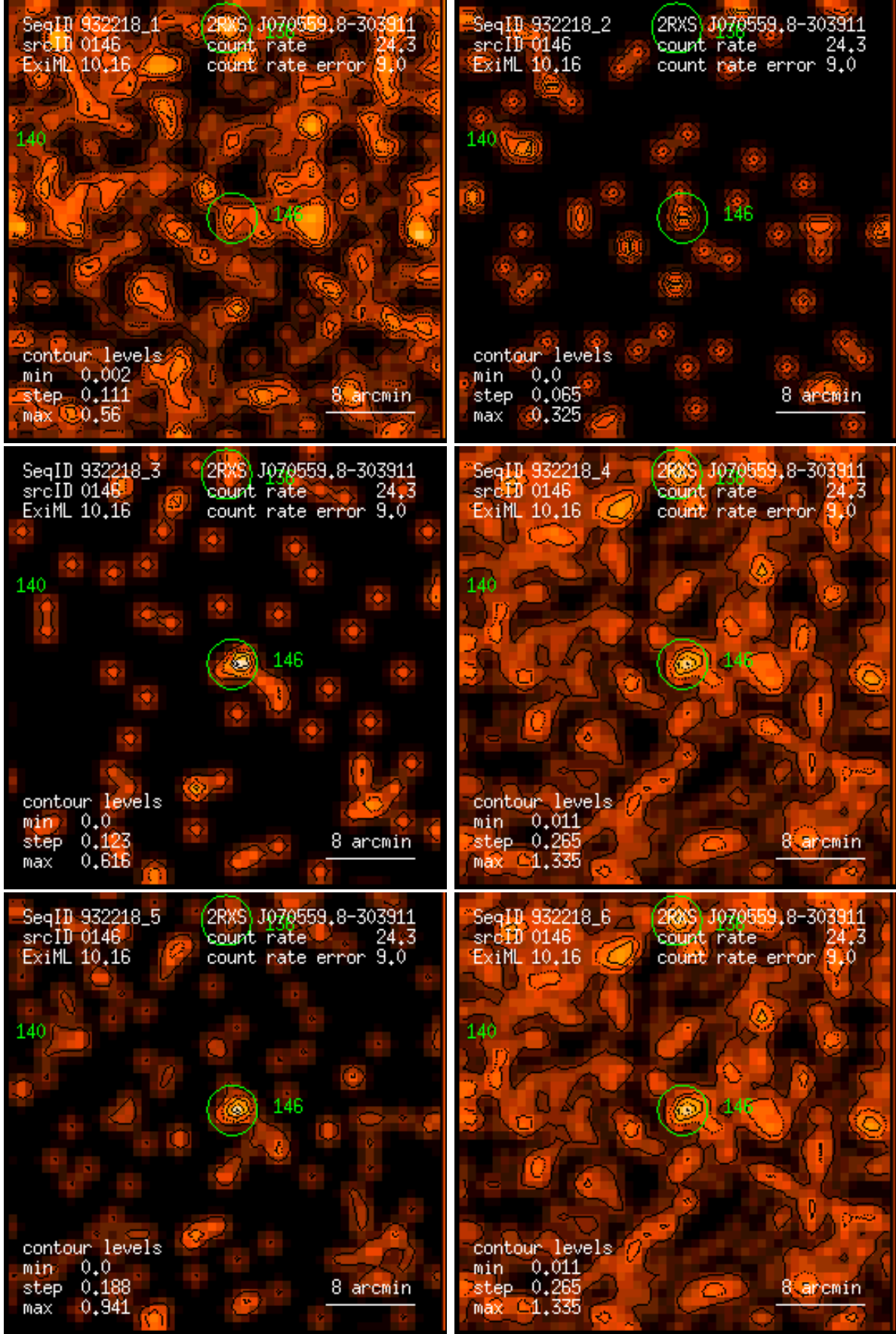
Figure 146: RASS 932218: detection 0146: band rate images, Gaussian filter: (1) PSPC channels 11 – 41, (2) 52 – 90, (3) 91 – 201, (4) 11 – 235, (5) 52 – 201, (6) 11 – 201. Broad band rates in counts/ks. Band rate contour levels in counts/ks/arcmin 2 .
