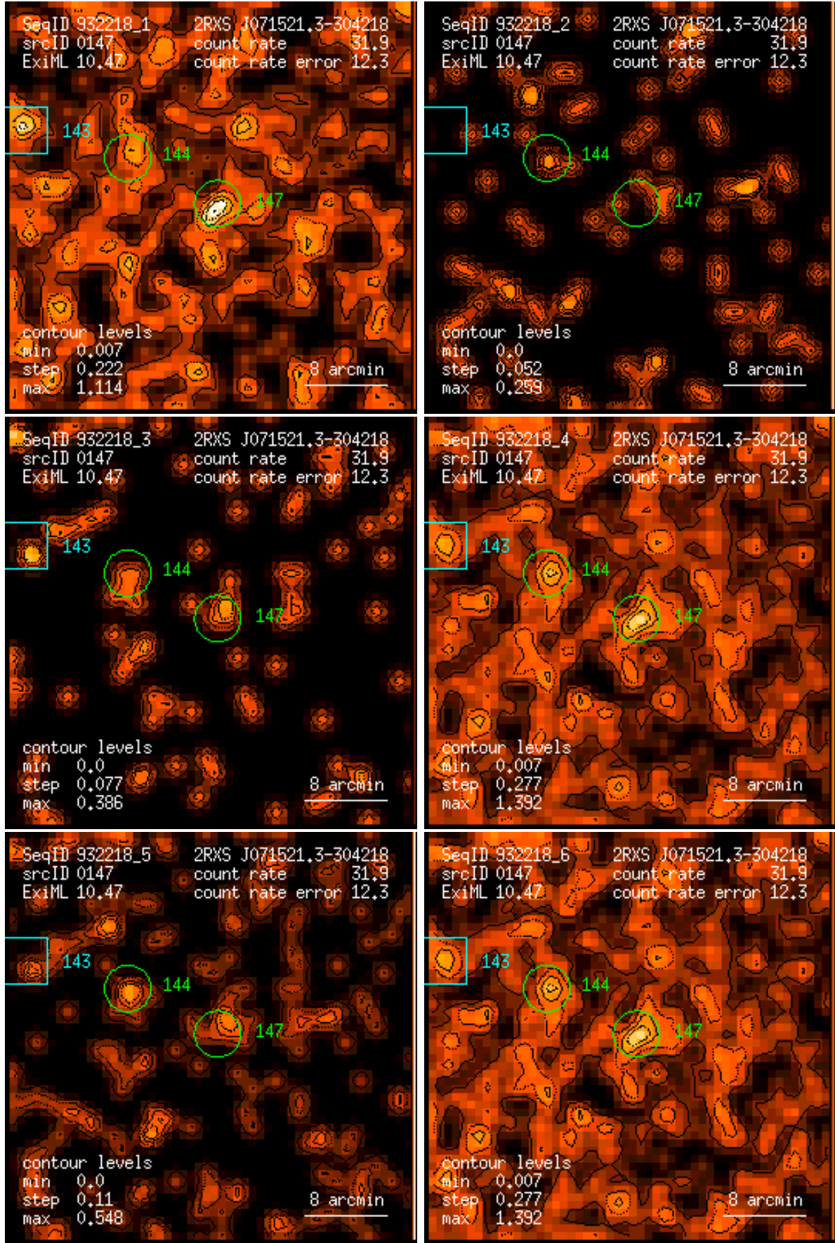
Figure 147: RASS 932218: detection 0147: band rate images, Gaussian filter: (1) PSPC channels 11 – 41, (2) 52 – 90, (3) 91 – 201, (4) 11 – 235, (5) 52 – 201, (6) 11 – 201. Broad band rates in counts/ks. Band rate contour levels in counts/ks/arcmin 2 .
