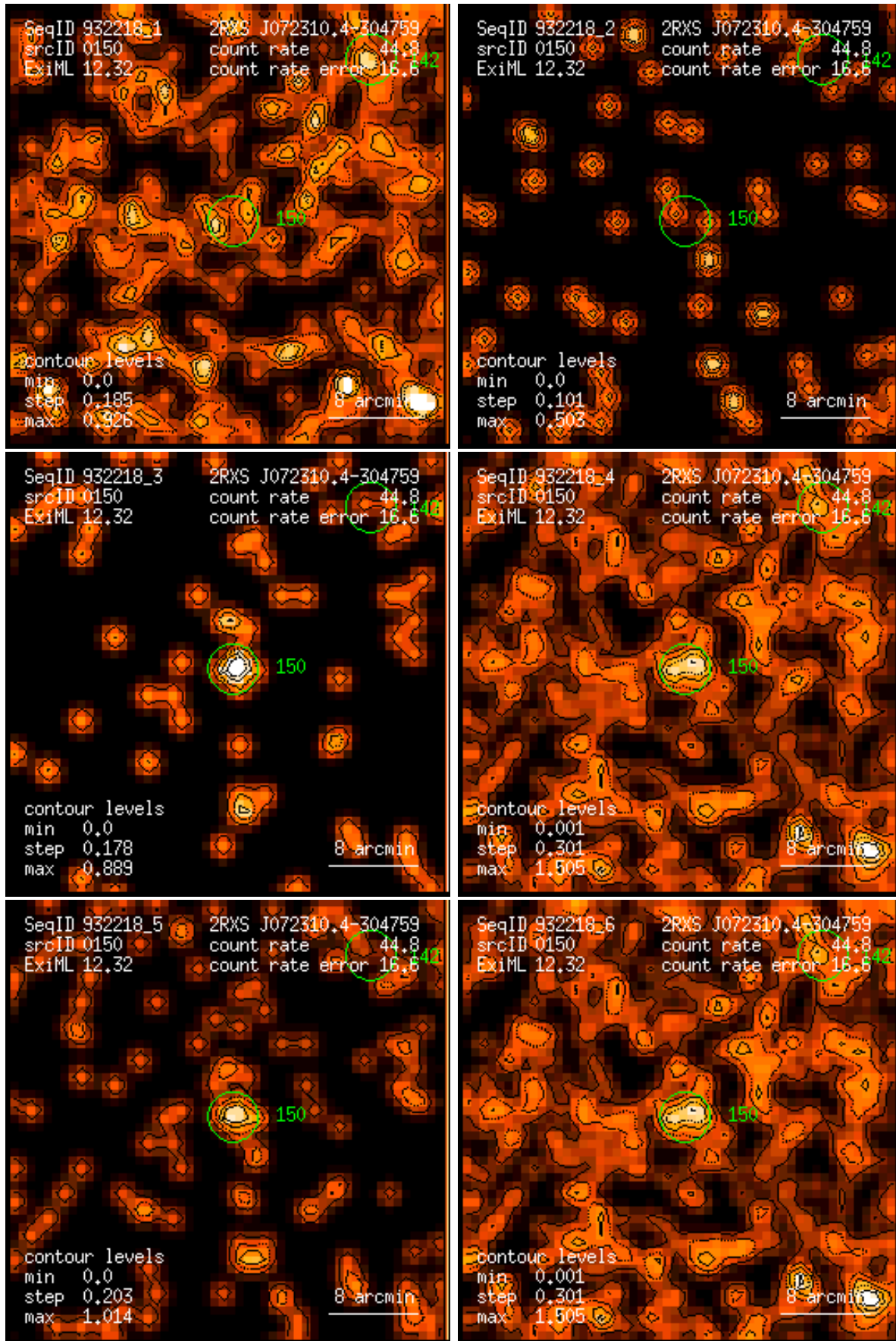
Figure 150: RASS 932218: detection 0150: band rate images, Gaussian filter: (1) PSPC channels 11 – 41, (2) 52 – 90, (3) 91 – 201, (4) 11 – 235, (5) 52 – 201, (6) 11 – 201. Broad band rates in counts/ks. Band rate contour levels in counts/ks/arcmin 2 .
