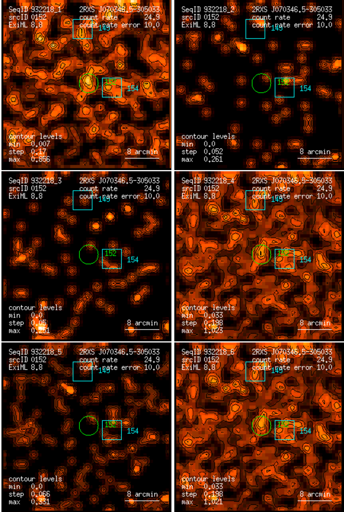
Figure 152: RASS 932218: detection 0152: band rate images, Gaussian filter: (1) PSPC channels 11 – 41, (2) 52 – 90, (3) 91 – 201, (4) 11 – 235, (5) 52 – 201, (6) 11 – 201. Broad band rates in counts/ks. Band rate contour levels in counts/ks/arcmin 2 .
