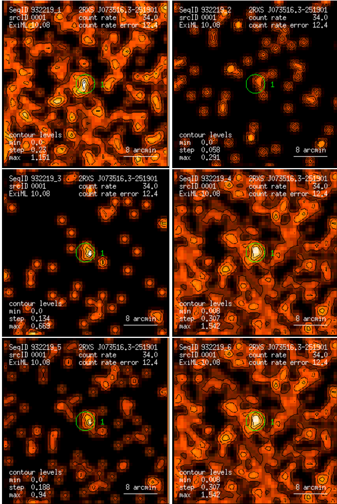
Figure 1: RASS 932219: detection 0001: band rate images, Gaussian filter: (1) PSPC channels 11 – 41, (2) 52 – 90, (3) 91 – 201, (4) 11 – 235, (5) 52 – 201, (6) 11 – 201. Broad band rates in counts/ks. Band rate contour levels in counts/ks/arcmin 2 .
