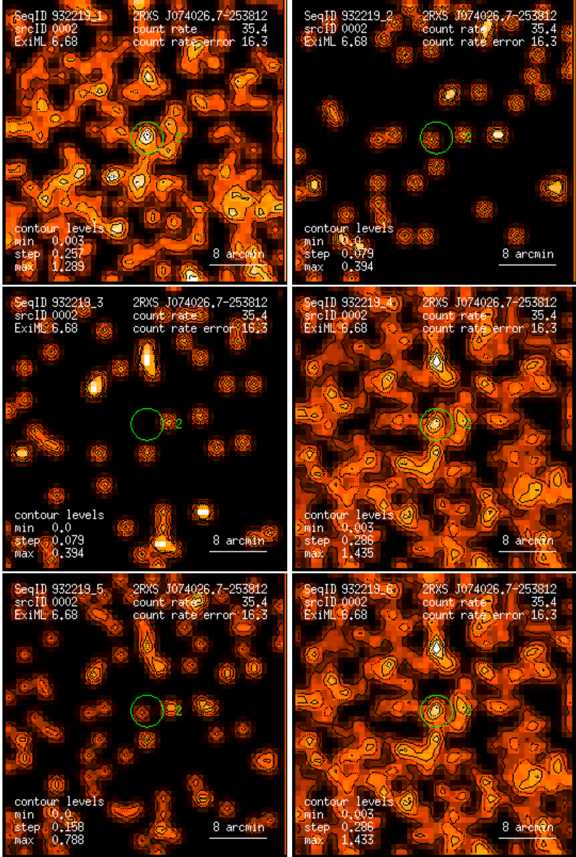
Figure 2: RASS 932219: detection 0002: band rate images, Gaussian filter: (1) PSPC channels 11 – 41, (2) 52 – 90, (3) 91 – 201, (4) 11 – 235, (5) 52 – 201, (6) 11 – 201. Broad band rates in counts/ks. Band rate contour levels in counts/ks/arcmin 2 .
