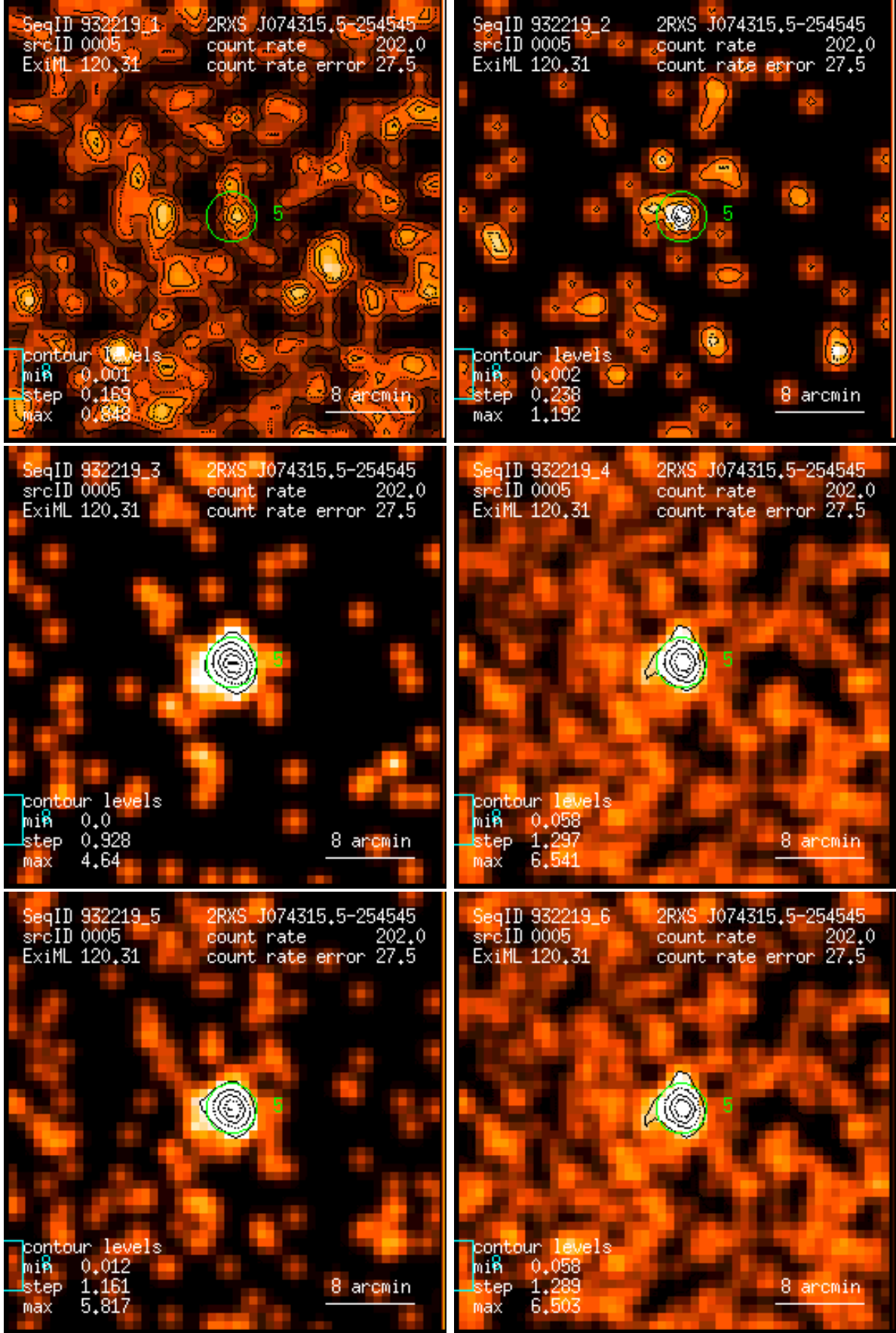
Figure 5: RASS 932219: detection 0005: band rate images, Gaussian filter: (1) PSPC channels 11 – 41, (2) 52 – 90, (3) 91 – 201, (4) 11 – 235, (5) 52 – 201, (6) 11 – 201. Broad band rates in counts/ks. Band rate contour levels in counts/ks/arcmin 2 .
