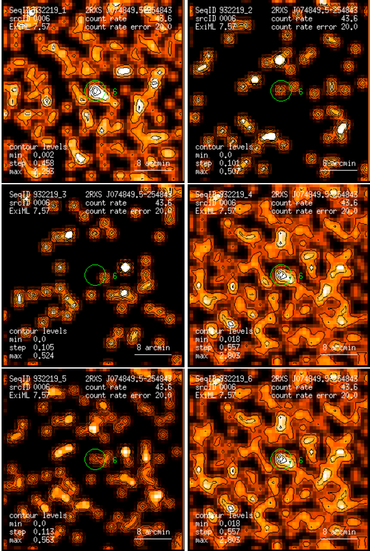
Figure 6: RASS 932219: detection 0006: band rate images, Gaussian filter: (1) PSPC channels 11 – 41, (2) 52 – 90, (3) 91 – 201, (4) 11 – 235, (5) 52 – 201, (6) 11 – 201. Broad band rates in counts/ks. Band rate contour levels in counts/ks/arcmin 2 .
