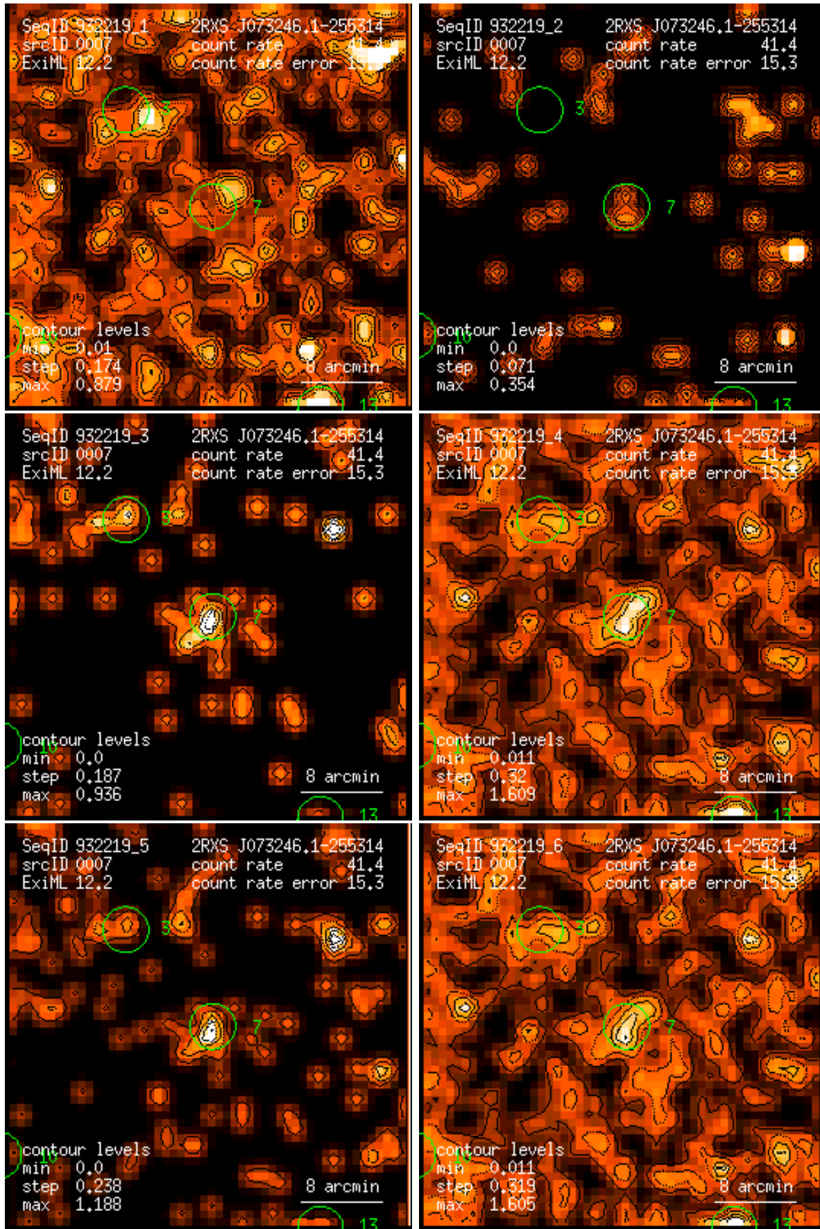
Figure 7: RASS 932219: detection 0007: band rate images, Gaussian filter: (1) PSPC channels 11 – 41, (2) 52 – 90, (3) 91 – 201, (4) 11 – 235, (5) 52 – 201, (6) 11 – 201. Broad band rates in counts/ks. Band rate contour levels in counts/ks/arcmin 2 .
