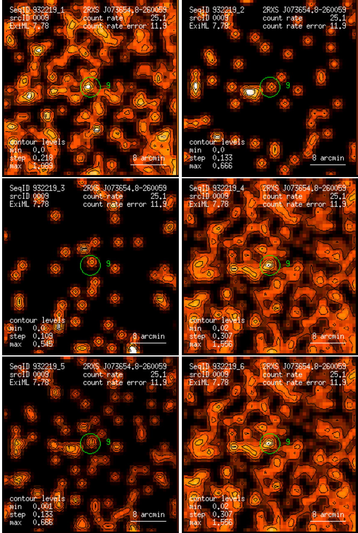
Figure 9: RASS 932219: detection 0009: band rate images, Gaussian filter: (1) PSPC channels 11 – 41, (2) 52 – 90, (3) 91 – 201, (4) 11 – 235, (5) 52 – 201, (6) 11 – 201. Broad band rates in counts/ks. Band rate contour levels in counts/ks/arcmin 2 .
