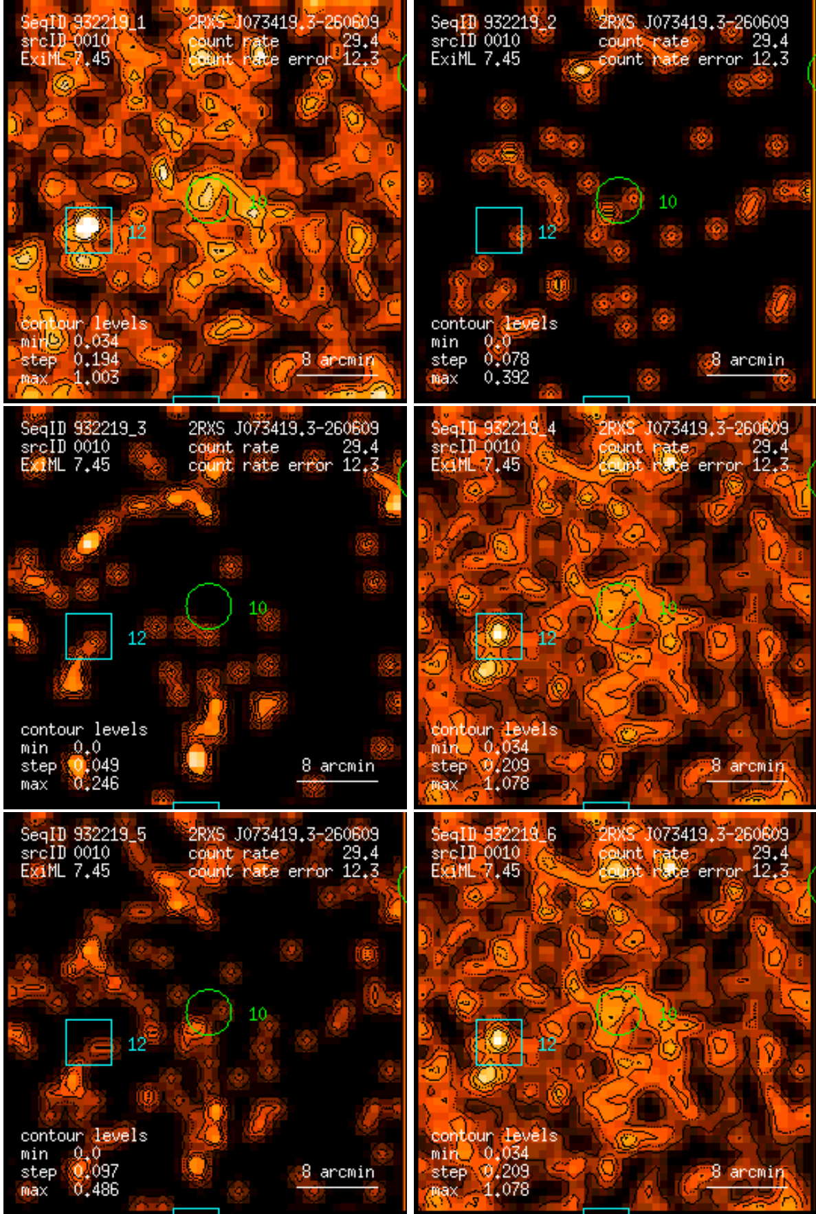
Figure 10: RASS 932219: detection 0010: band rate images, Gaussian filter: (1) PSPC channels 11 – 41, (2) 52 – 90, (3) 91 – 201, (4) 11 – 235, (5) 52 – 201, (6) 11 – 201. Broad band rates in counts/ks. Band rate contour levels in counts/ks/arcmin 2 .
