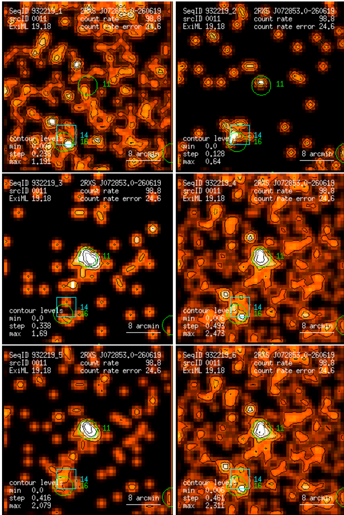
Figure 11: RASS 932219: detection 0011: band rate images, Gaussian filter: (1) PSPC channels 11 – 41, (2) 52 – 90, (3) 91 – 201, (4) 11 – 235, (5) 52 – 201, (6) 11 – 201. Broad band rates in counts/ks. Band rate contour levels in counts/ks/arcmin 2 .
