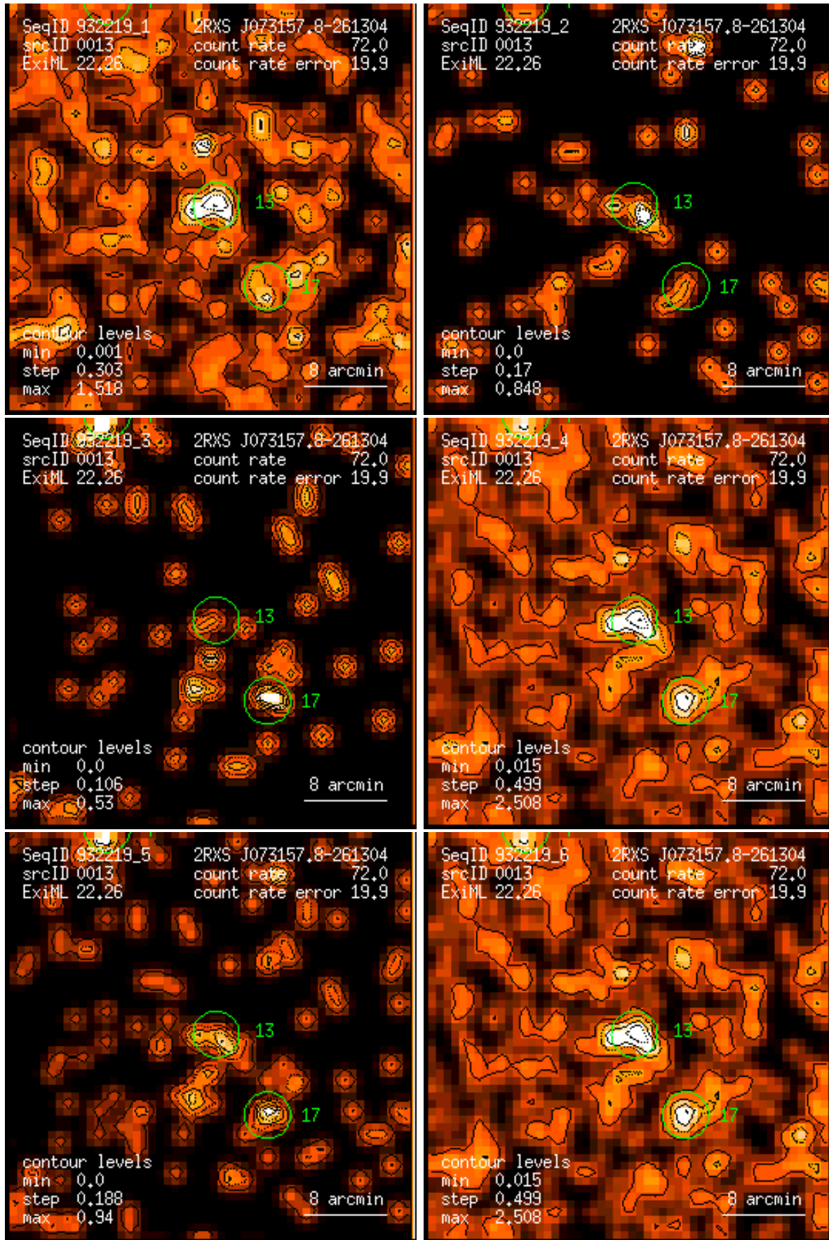
Figure 13: RASS 932219: detection 0013: band rate images, Gaussian filter: (1) PSPC channels 11 – 41, (2) 52 – 90, (3) 91 – 201, (4) 11 – 235, (5) 52 – 201, (6) 11 – 201. Broad band rates in counts/ks. Band rate contour levels in counts/ks/arcmin 2 .
