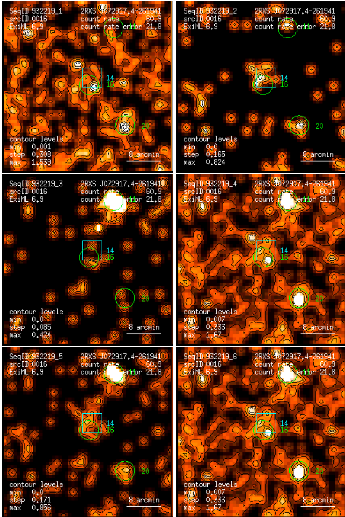
Figure 16: RASS 932219: detection 0016: band rate images, Gaussian filter: (1) PSPC channels 11 – 41, (2) 52 – 90, (3) 91 – 201, (4) 11 – 235, (5) 52 – 201, (6) 11 – 201. Broad band rates in counts/ks. Band rate contour levels in counts/ks/arcmin 2 .
