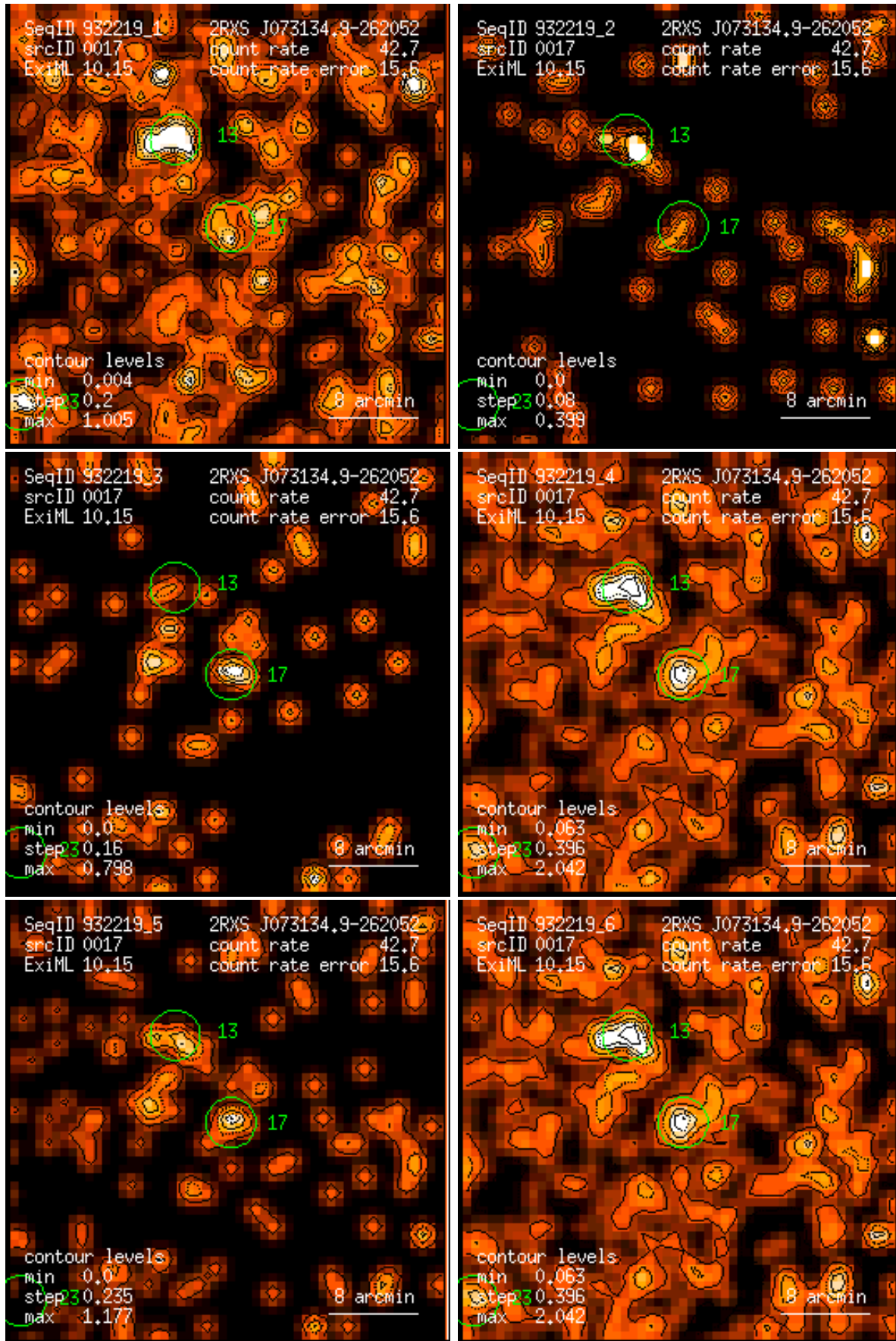
Figure 17: RASS 932219: detection 0017: band rate images, Gaussian filter: (1) PSPC channels 11 – 41, (2) 52 – 90, (3) 91 – 201, (4) 11 – 235, (5) 52 – 201, (6) 11 – 201. Broad band rates in counts/ks. Band rate contour levels in counts/ks/arcmin 2 .
