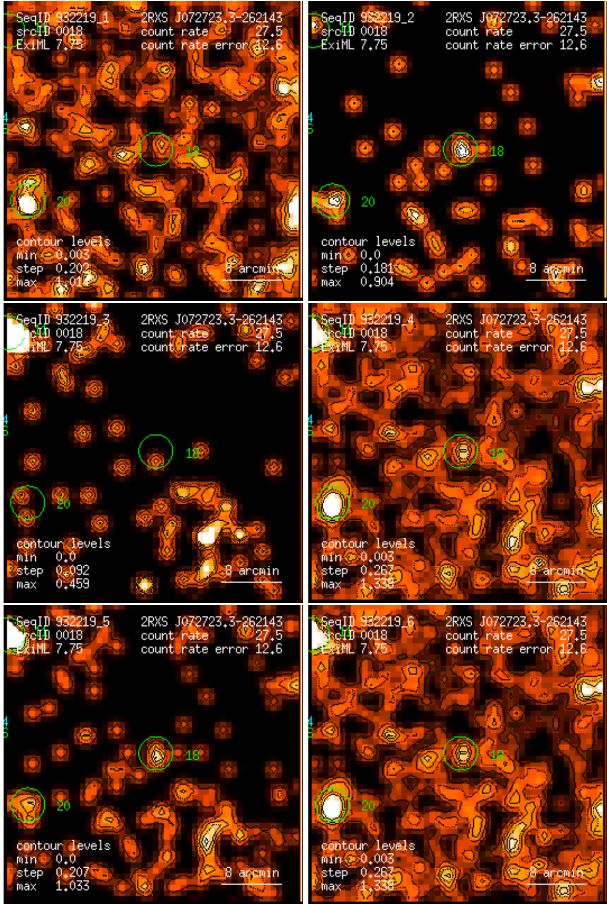
Figure 18: RASS 932219: detection 0018: band rate images, Gaussian filter: (1) PSPC channels 11 – 41, (2) 52 – 90, (3) 91 – 201, (4) 11 – 235, (5) 52 – 201, (6) 11 – 201. Broad band rates in counts/ks. Band rate contour levels in counts/ks/arcmin 2 .
