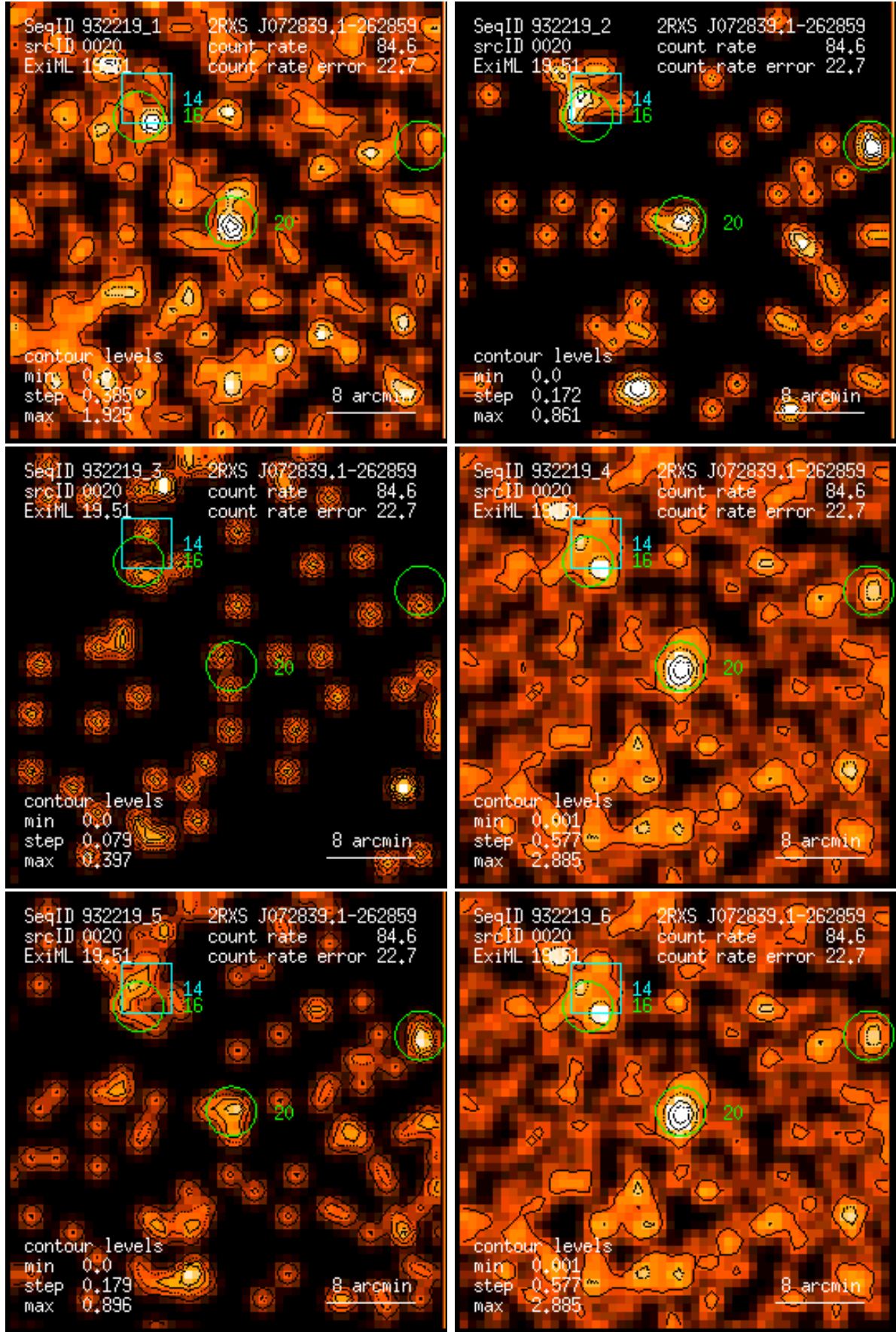
Figure 20: RASS 932219: detection 0020: band rate images, Gaussian filter: (1) PSPC channels 11 – 41, (2) 52 – 90, (3) 91 – 201, (4) 11 – 235, (5) 52 – 201, (6) 11 – 201. Broad band rates in counts/ks. Band rate contour levels in counts/ks/arcmin 2 .
