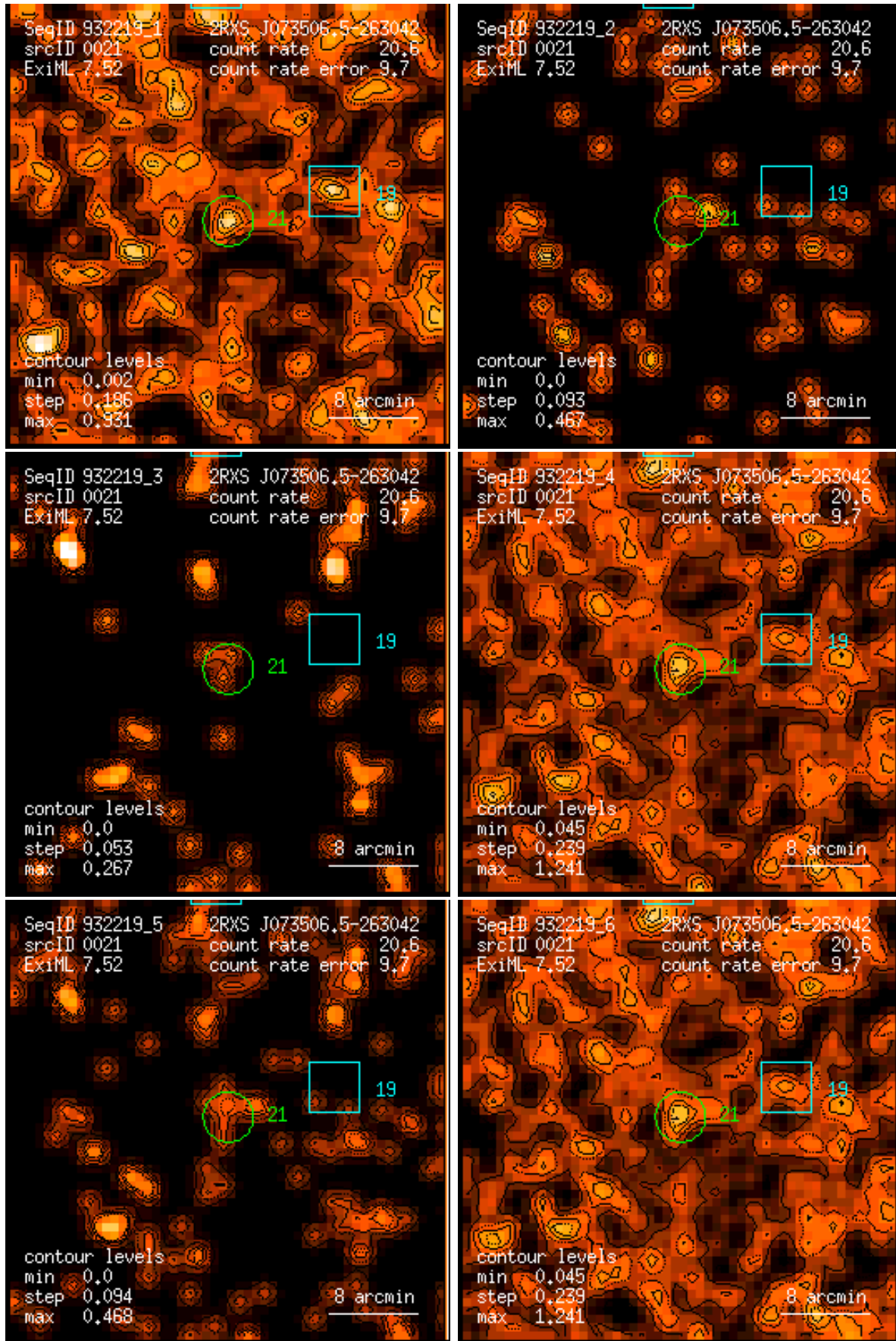
Figure 21: RASS 932219: detection 0021: band rate images, Gaussian filter: (1) PSPC channels 11 – 41, (2) 52 – 90, (3) 91 – 201, (4) 11 – 235, (5) 52 – 201, (6) 11 – 201. Broad band rates in counts/ks. Band rate contour levels in counts/ks/arcmin 2 .
