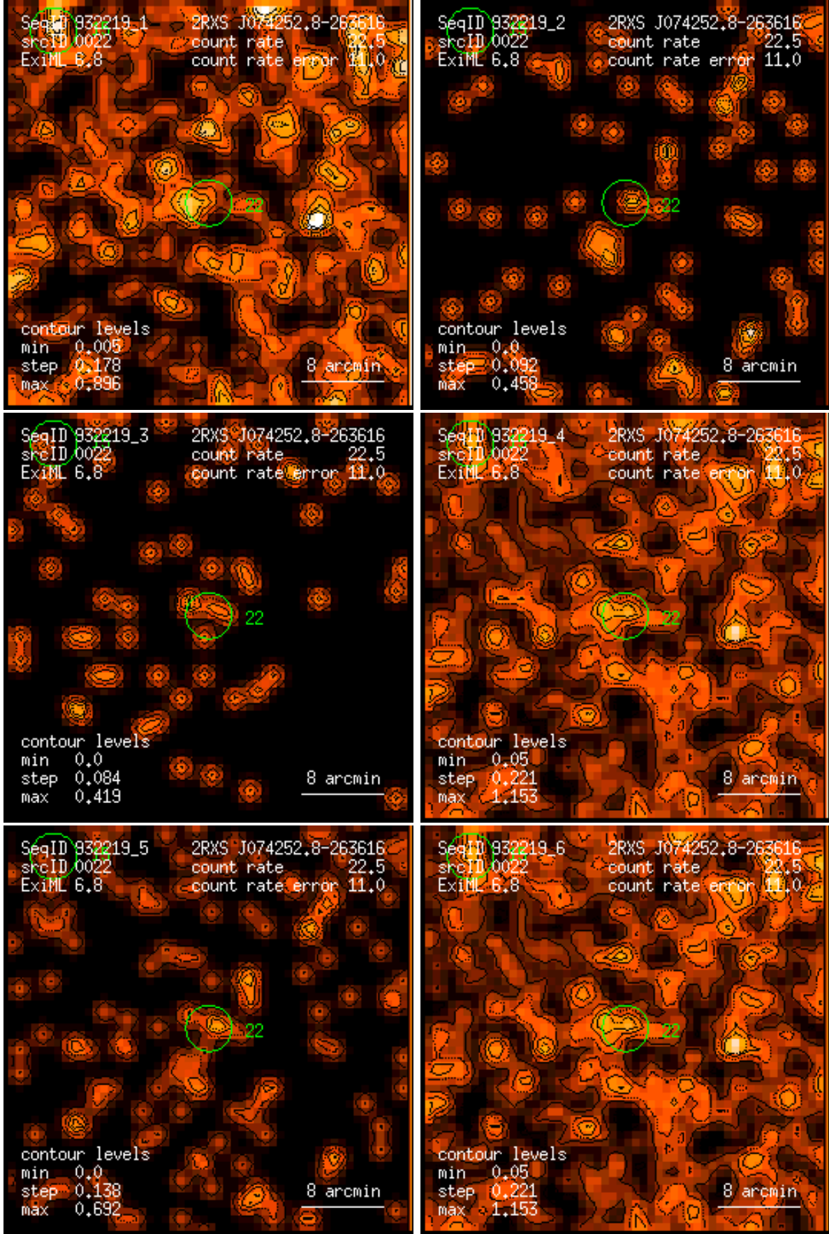
Figure 22: RASS 932219: detection 0022: band rate images, Gaussian filter: (1) PSPC channels 11 – 41, (2) 52 – 90, (3) 91 – 201, (4) 11 – 235, (5) 52 – 201, (6) 11 – 201. Broad band rates in counts/ks. Band rate contour levels in counts/ks/arcmin 2 .
