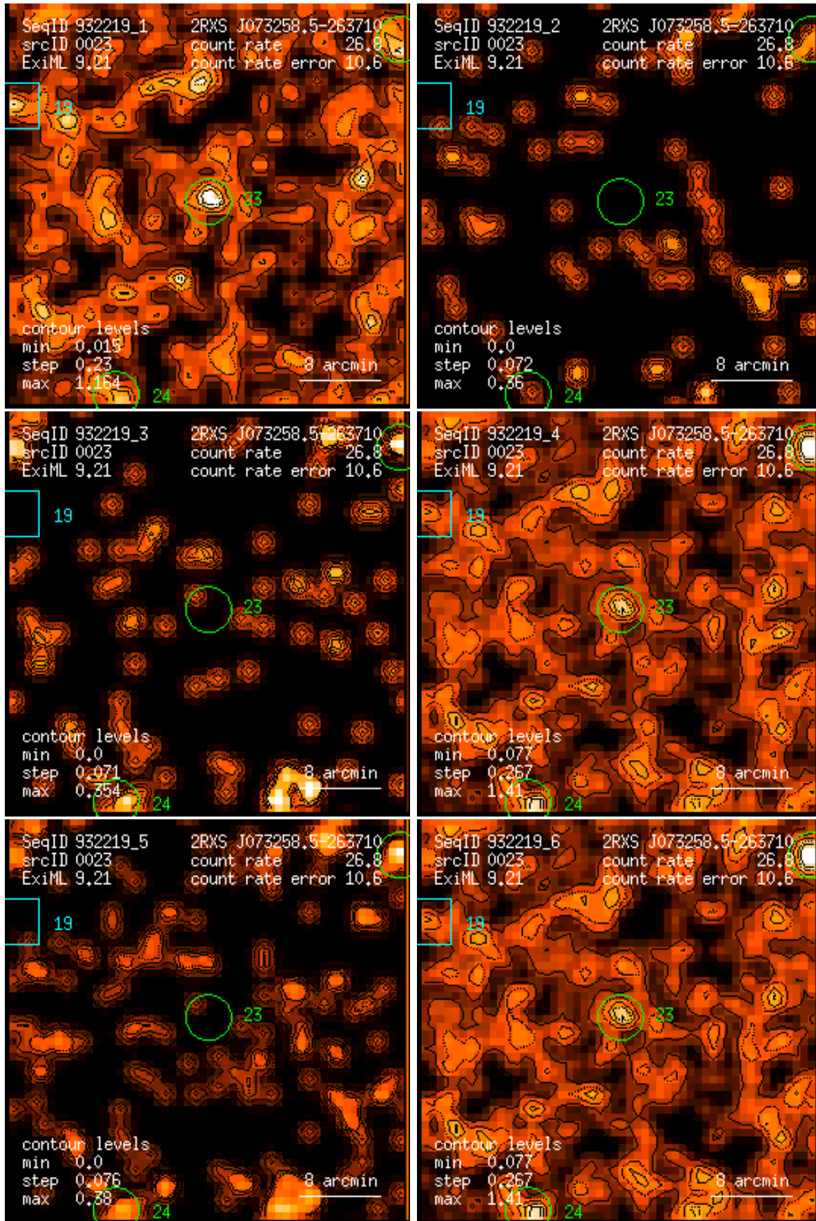
Figure 23: RASS 932219: detection 0023: band rate images, Gaussian filter: (1) PSPC channels 11 – 41, (2) 52 – 90, (3) 91 – 201, (4) 11 – 235, (5) 52 – 201, (6) 11 – 201. Broad band rates in counts/ks. Band rate contour levels in counts/ks/arcmin 2 .
