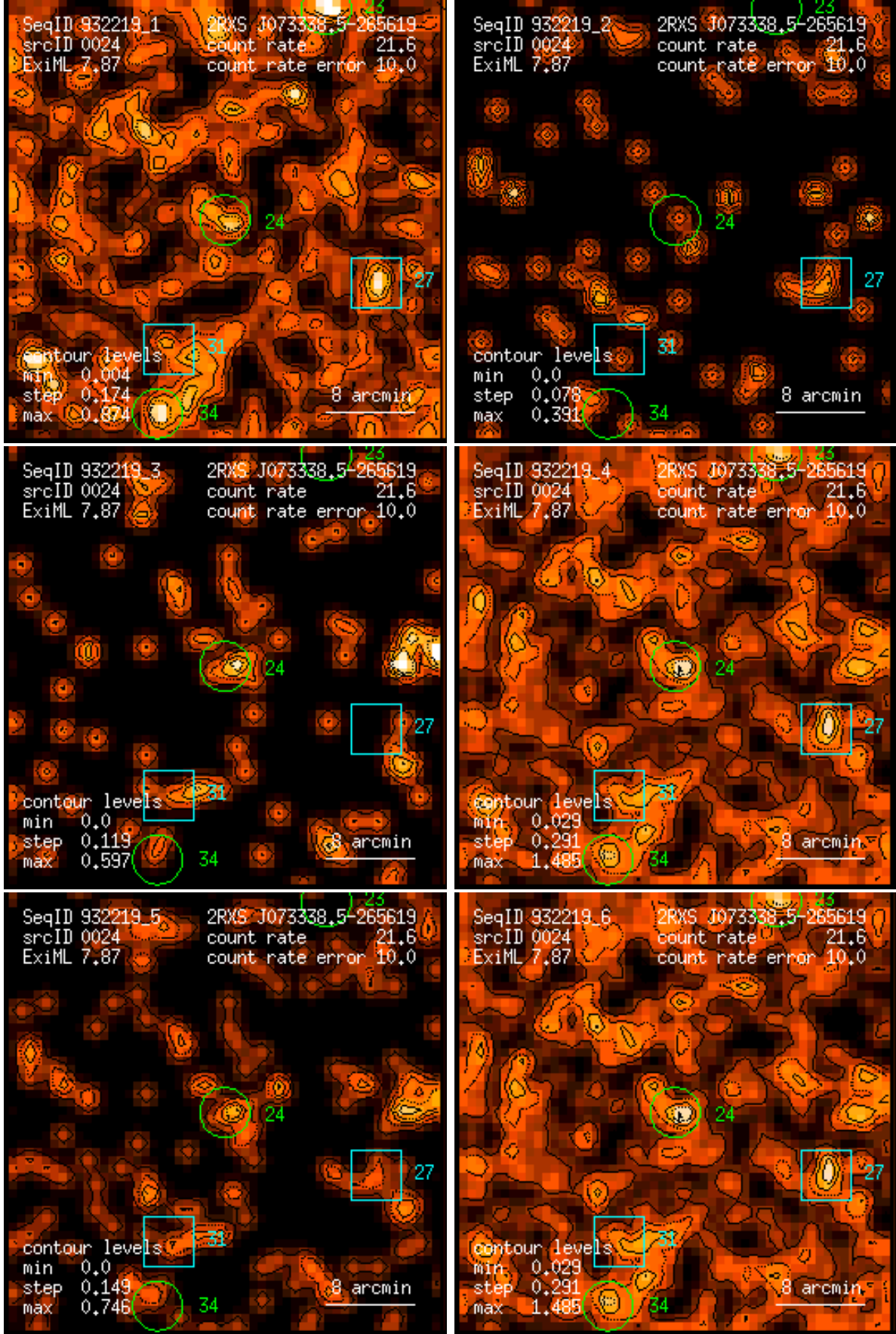
Figure 24: RASS 932219: detection 0024: band rate images, Gaussian filter: (1) PSPC channels 11 – 41, (2) 52 – 90, (3) 91 – 201, (4) 11 – 235, (5) 52 – 201, (6) 11 – 201. Broad band rates in counts/ks. Band rate contour levels in counts/ks/arcmin 2 .
