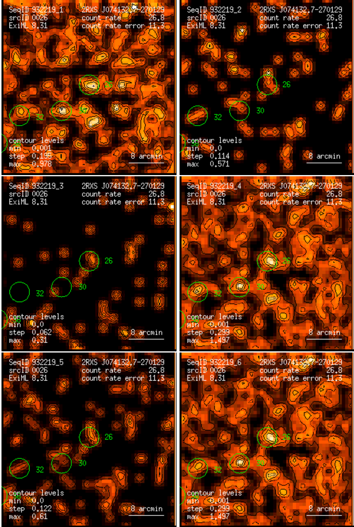
Figure 26: RASS 932219: detection 0026: band rate images, Gaussian filter: (1) PSPC channels 11 – 41, (2) 52 – 90, (3) 91 – 201, (4) 11 – 235, (5) 52 – 201, (6) 11 – 201. Broad band rates in counts/ks. Band rate contour levels in counts/ks/arcmin 2 .
