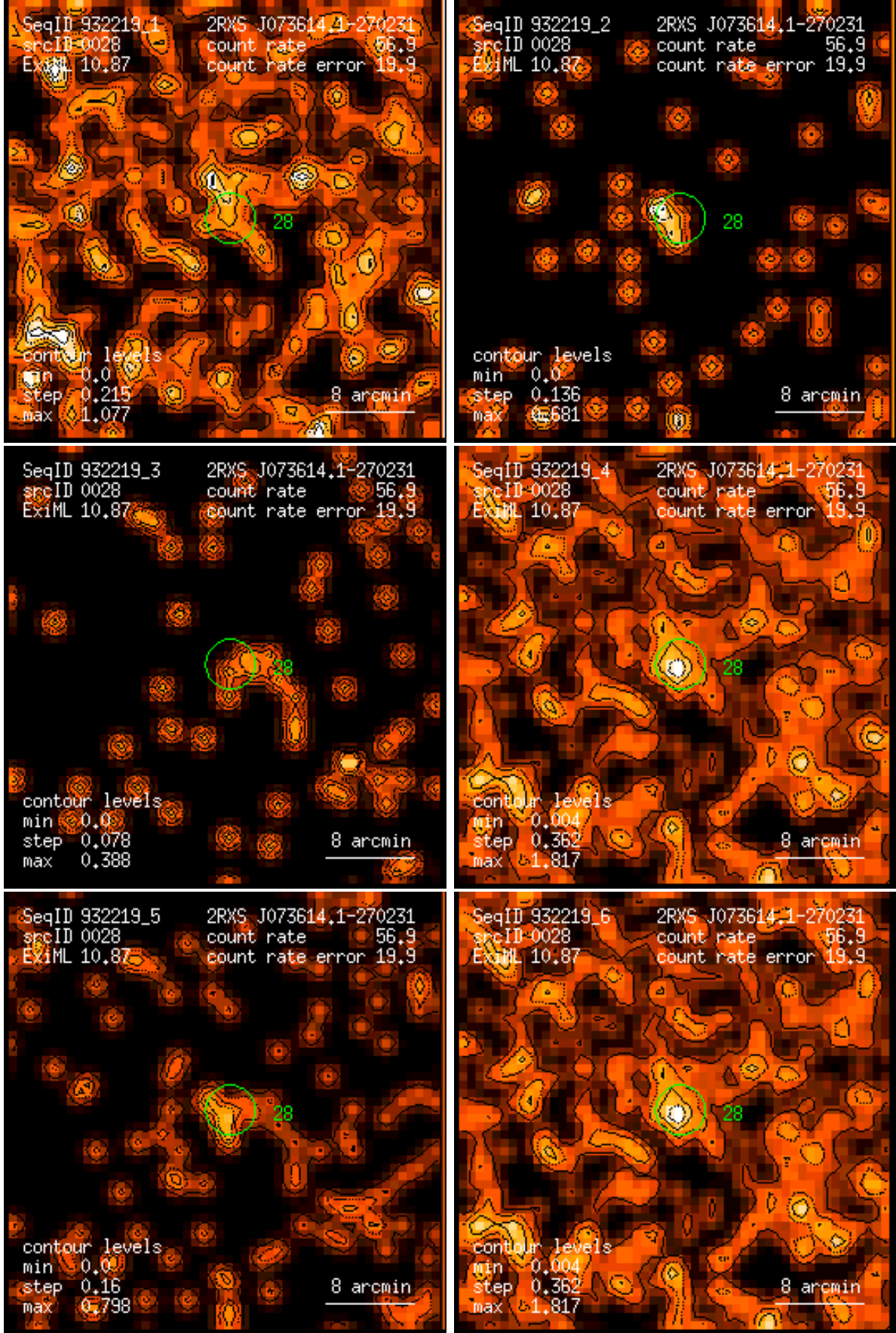
Figure 28: RASS 932219: detection 0028: band rate images, Gaussian filter: (1) PSPC channels 11 – 41, (2) 52 – 90, (3) 91 – 201, (4) 11 – 235, (5) 52 – 201, (6) 11 – 201. Broad band rates in counts/ks. Band rate contour levels in counts/ks/arcmin 2 .
